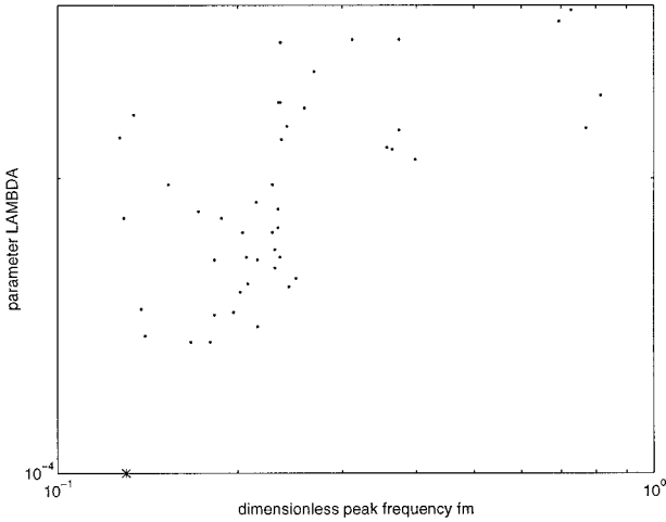
FIG. 6. Values of parameter \lambda (37) versus dimensionless peak frequency \tilde{f}_m .
