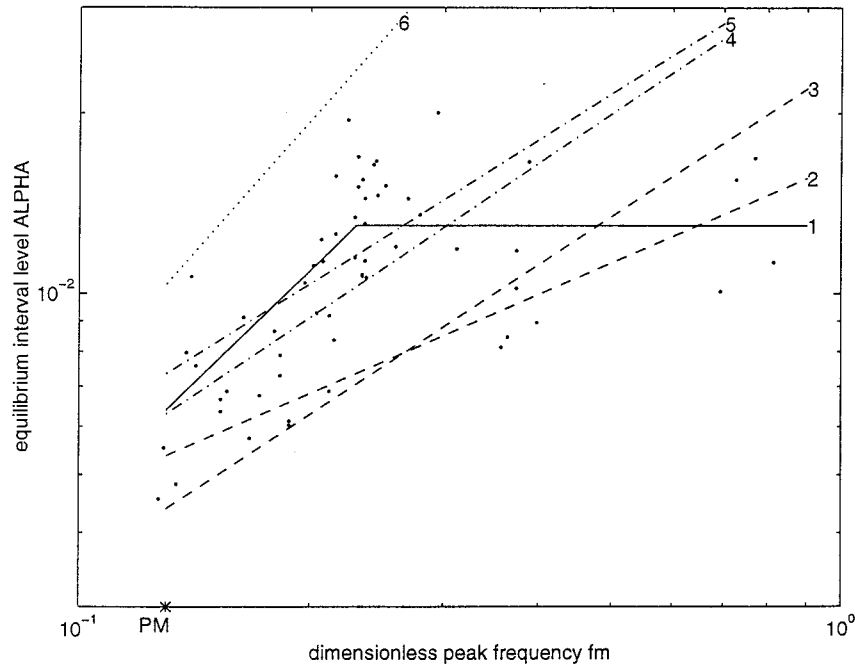
FIG. 5. Dependencies of equilibrium interval spectral density level \alpha on dimensionless peak frequency \tilde{f}_m : the solid line numbered 1 is dependence (25), dependencies numbered 2–6 are 2: Donelan et al.'s (26), 3: Evans and Kibblewhite's (27), 4: Bandou et al.'s (28), 5: JONSWAP's with the laboratory data (31), and 6: JONSWAP's without the laboratory data (32). PM is the Pierson–Moskowitz frequency.
