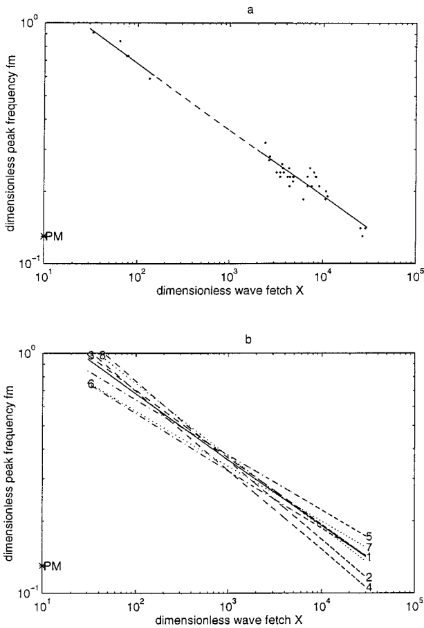
FIG. 3. (a) Dependence (8) of dimensionless peak frequency \tilde{f}_m on dimensionless fetch X ; (b) comparison of the dimensionless peak frequency \tilde{f}_m on the dimensionless fetch X dependency: the solid line numbered 1 is our dependence (8), dependencies numbered 2–8 are 2: JONSWAP’s (1), 3: Davidan’s (2), 4: Kahma’s (3), 5: Donelan et al.’s (4), 6: Dobson et al.’s (5), 7: Wen’s et al.’s (6), and 8: Evans and Kibblewhite’s (7). PM is the Pierson–Moskowitz frequency.
