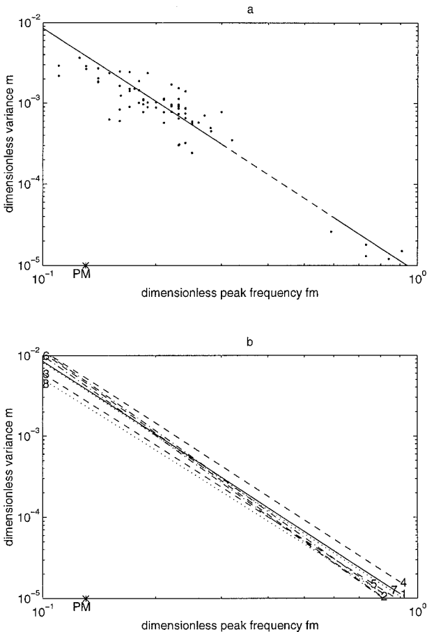
FIG. 4. (a) Dependence (10) of dimensionless wave variance \tilde{m} on dimensionless peak frequency \tilde{f}_m ; (b) comparison of the dimensionless wave variance \tilde{m} on the dimensionless peak frequency \tilde{f}_m dependency: the solid line numbered 1 is our dependence (10), dependencies numbered 2–8 are 2: Hasselmann et al.'s (11), 3: Davidan's (12), 4: Kahma's (13), 5: Donelan et al.'s (14), 6: Dobson et al.'s (15), 7: Wen et al.'s (16), and 8: Evans and Kibblewhite's (17). PM is the Pierson–Moskowitz frequency.
