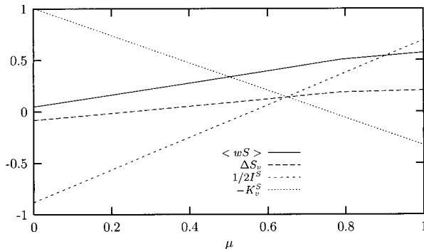
Fig. 11. Saline component of the buoyancy production \langle wS \rangle and its components as a function of the parameter \mu , where \mu = 0 denotes the model with the total salt flux prescribed, whereas at \mu = 1 the zonally averaged overturning component is prescribed (see Fig. 4). Note that an increase in \langle wS \rangle corresponds to an increase in the weakening effect of salinity on the circulation strength (a decrease in \langle wB \rangle ).
