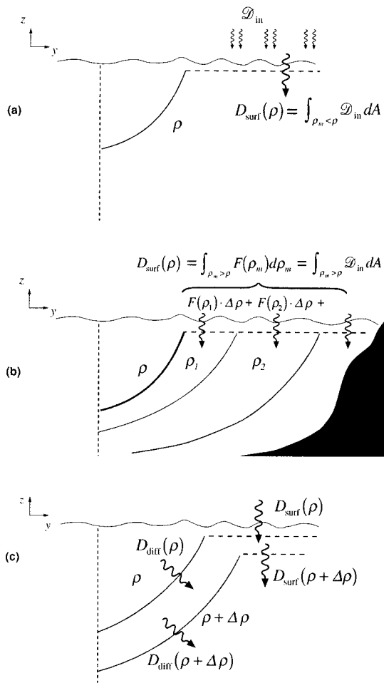
FIG. 3. (a) A schematic vertical section showing the \rho isopycnal (solid line) and its surface extension (dotted line). The surface extension lies along the sea surface wherever the isopycnal is lighter than the surface mixed layer water \rho < \rho_m(\mathbf{x}) . The density flux through the surface extension is then D_{\text{surf}} = \int_{\rho_m < \rho} \mathcal{D}_{\text{in}} dA . (b) The density flux D_{\text{surf}}(\rho) through the surface extension is made up of the surface fluxes F into all the outcropping isopycnals denser than \rho . Here \rho_1 = \rho + \frac{1}{2}\Delta\rho , \rho_2 = \rho + \frac{3}{2}\Delta\rho , etc. (c) A control volume between the \rho and \rho + \Delta\rho isopycnals and their surface extensions, showing the diffusive and surface fluxes into and out of it.
