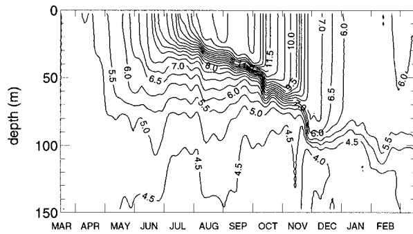
FIG. 1. The annual cycle at OWS Papa (50°N, 145°W) of the depth profile of temperature in °C over the “ocean year” 15 March 1961 to 15 March 1962. Redrawn from Large et al. (1994).
