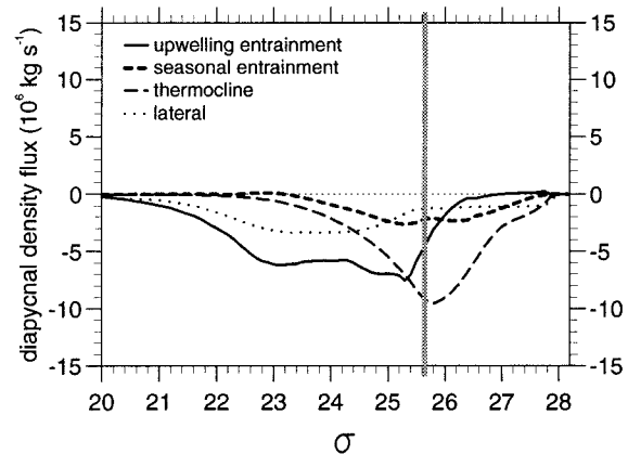
FIG. 12. Annual-mean basin-integrated interior diffusive flux D_{\text{diff}} separated into explicit thermocline diffusion D_{\text{thermo}} (thin dashed line), the entrainment flux from equatorial and eastern boundary upwelling regions D_{\text{equat}} (full line), the entrainment flux in the seasonal boundary layer D_{\text{seas}} (thick dashed line), and the horizontal diffusive flux within the mixed layer D_{\text{lat}} (dotted line). Units are 10^6 \text{ kg s}^{-1} .
