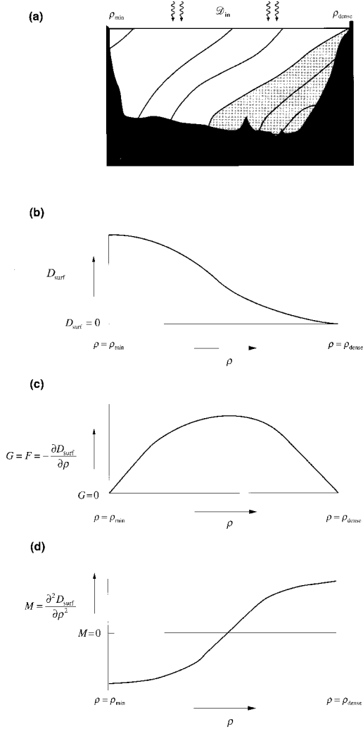
FIG. 4. (a) Schematic section through an idealized basin with surface density gain and no mixing. The lightest water in the basin has density \rho_{min} and \rho_{dense} is the densest water that outcrops; water denser than \rho_{dense} is shaded. (b) The variation of the surface-integrated density flux D_{surf}(\rho) with \rho , (c) the implied diapycnal volume flux G(\rho) = F = -\partial D_{surf}/\partial \rho , and (d) the water mass formation rate M(\rho) = -\partial G/\partial \rho . In this example, the surface density input drives a diapycnal volume flux toward denser waters in (c), which leads to the densest waters being formed at the expense of the lightest waters in (d).
