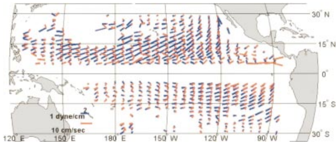
FIG. 1. The mean wind stress and ageostrophic force as measured by the drifters and binned into 2^\circ \times 5^\circ boxes.
