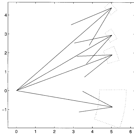
FIG. 5. Each arrow is the mean velocity vector within a depth range of z_0/H_* , where H_* \propto u_* f^{-1/2} . The amplitudes have been scaled by \beta u_* f^{-1/2} . The rotation to the right increases as z_0/H_* deepens. The dashed boxes around the arrowheads indicate the confidence intervals in the magnitude and rotation.
