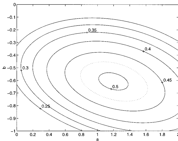
FIG. 2. A comparison of R^2 , percent of variance accounted for as a function of a and b , the exponents in the model \beta u_*^a f^b of the ageostrophic velocity.
