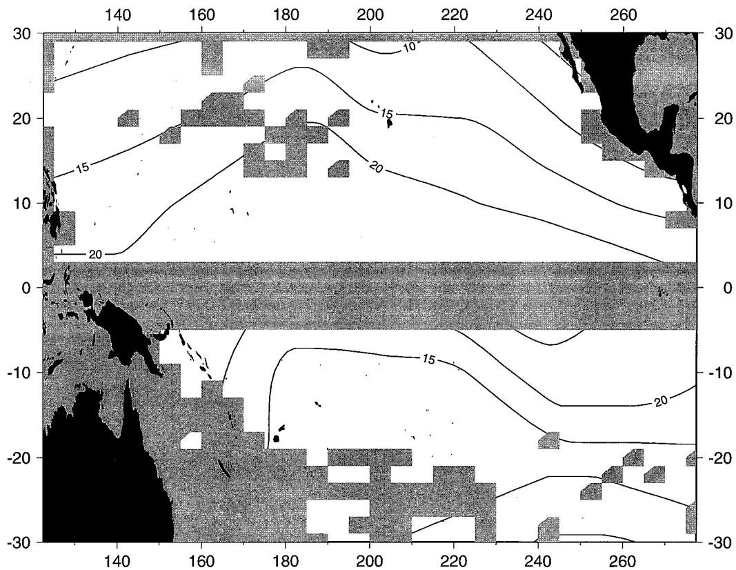
FIG. 4. The modeled Ekman depth based upon the scaling, H_* \propto u_* f^{-1/2} .
