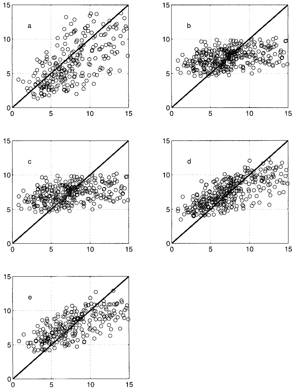
FIG. 3. Ageostrophic velocity magnitude (ordinate) vs modeled velocity (abscissa). (a) Model 1: u_*^2/(fD_T) ; (b) model 2: u_* ; (c) model 3: u_*^2 f^{-1/2} ; (d) model 4: u_* f^{-1/2} ; and (e) model 5: u_*/(N/f)^{1/2} .
