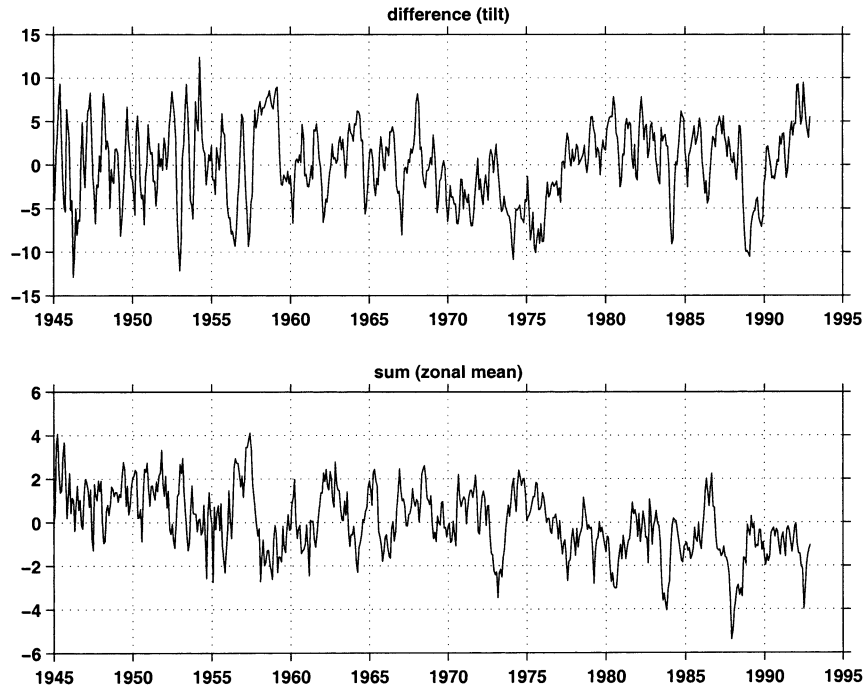
FIG. 4. The difference and sum of the TDA in the Niño-3 region (5°N/S, 90°–150°W) and the western warm pool (5°N/S, 120°E–180°) of the equatorial Pacific. The difference is defined as \frac{1}{2}(TDA_{\text{Niño}} - TDA_{\text{wp}}) and represents the tilt of the equatorial thermocline. Units are in meters. The sum is defined as \frac{1}{2}(TDA_{\text{Niño}} + TDA_{\text{wp}}) and represents zonal mean changes in the depth of the equatorial thermocline.
