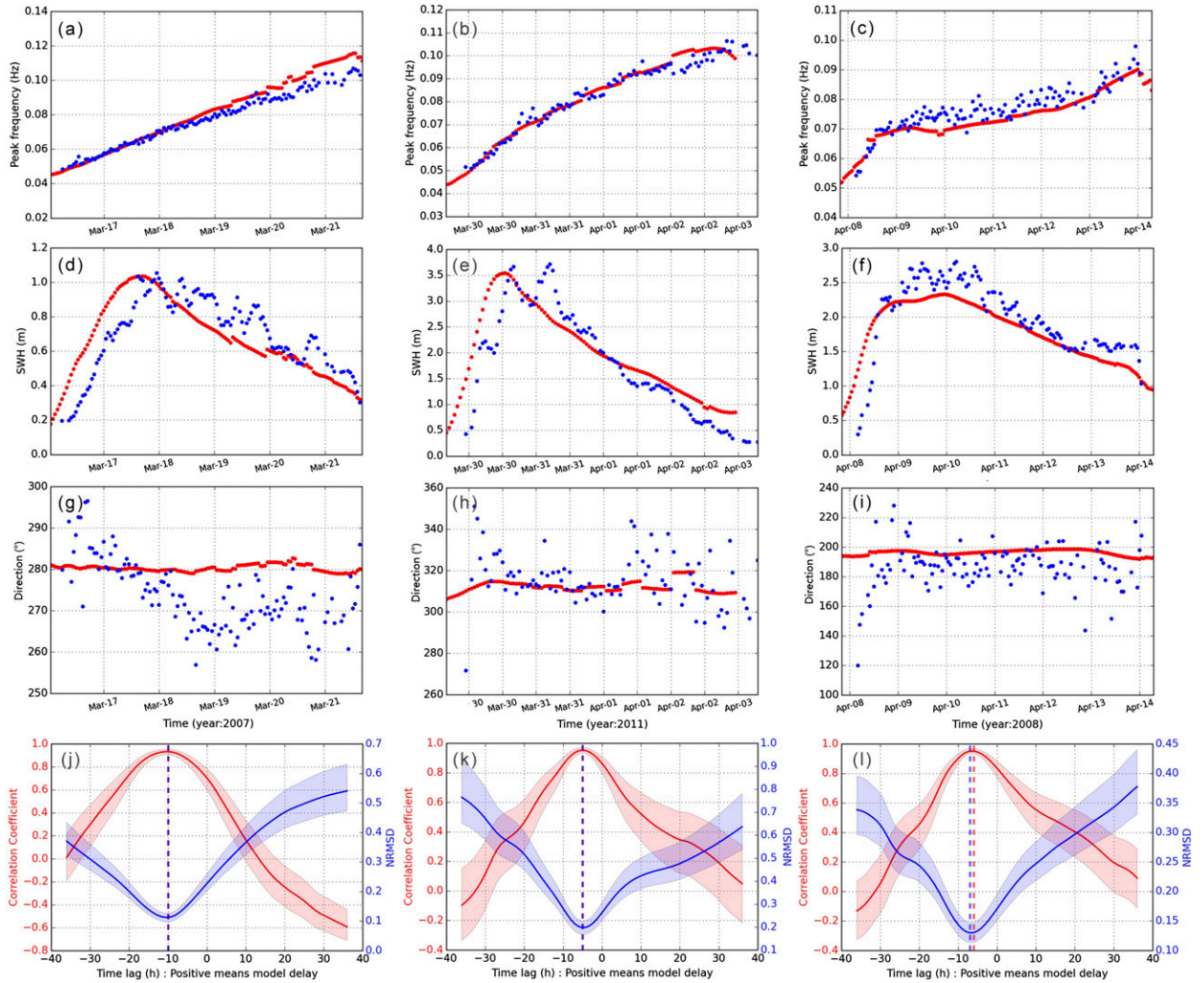
FIG. 1. (a)–(c) Peak frequencies, (d)–(f) wave heights, (g)–(i) peak directions, and (j)–(l) arrival time differences of collocated swell events from NDBC platform (left) 46086 in 2007, (center) 51101 in 2011, and (right) 32012 in 2008; in the first three rows, the blue dots are buoy measurements and the red dots are model outputs. In the fourth row, the red lines are the moving correlation coefficients and the blue lines are the moving NRMSDs [see Eqs. (1) and (2) for the definitions], and the shadow areas represent the 95% confidence intervals. The respective dot vertical lines are where the maximum of moving correlation coefficients and the minimum of moving NRMSDs appear.
