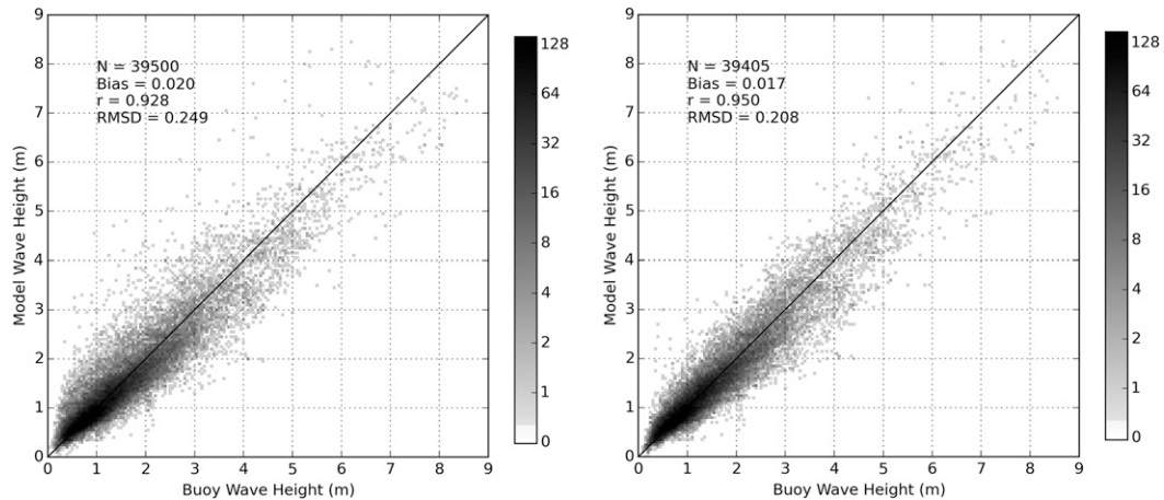
FIG. 3. The scatterplot of collocated wave heights of WW3 hindcast against NDBC buoys for the 421 swell events (a) without any correction and (b) after shifting the wave heights sequence with the arrival time difference.
