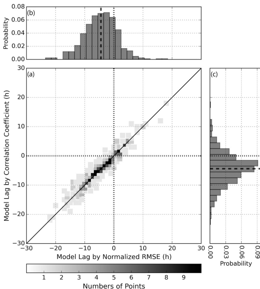
FIG. 2. (a) The scatterplot of the arrival time differences defined by shifting NRMSD vs those defined by cross correlation; (b),(c) respective histograms of arrival time differences.
