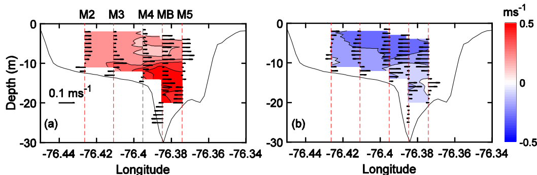
FIG. 5. Cross-channel distributions of the along-channel (color) and lateral (horizontal black lines) velocities during (a) flood and (b) ebb tides, obtained from bottom-mounted ADCPs at the mooring stations.
