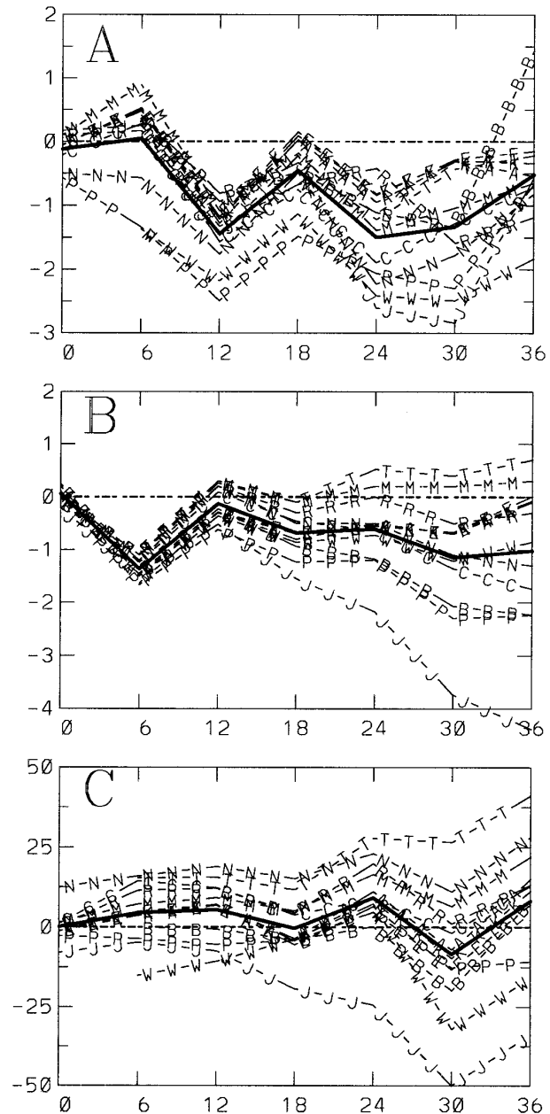
FIG. 13. Time series of bias, with respect to the RPN-prepared COMPARE analysis, for (a) 300-hPa wind speed ( \text{m s}^{-1} ), (b) 850-hPa temperature ( ^{\circ}\text{C} ), and (c) 300-hPa height (m) for E3 (50 km/18 levels) with the 12 participants (lettered) and composites (solid) shown. Data for the participants W, B, and T at the initial time are not available.
