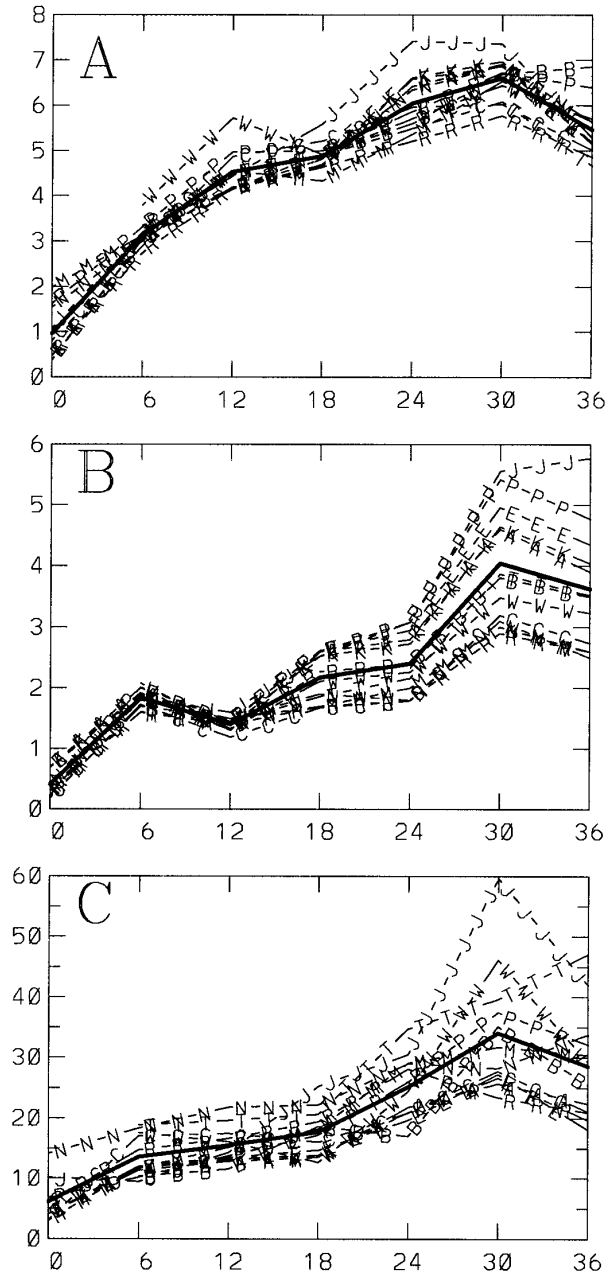
FIG. 12. Time series of rms errors, with respect to the RPN-prepared COMPARE analysis, for (a) 300-hPa wind speed ( \text{m s}^{-1} ), (b) 850-hPa temperature ( ^{\circ}\text{C} ), and (c) 300-hPa height (m) for E3 (50 km/18 levels) with the 12 participants (lettered) and composites (solid) shown. Data for the participants W, B, and T at the initial time are not available.
