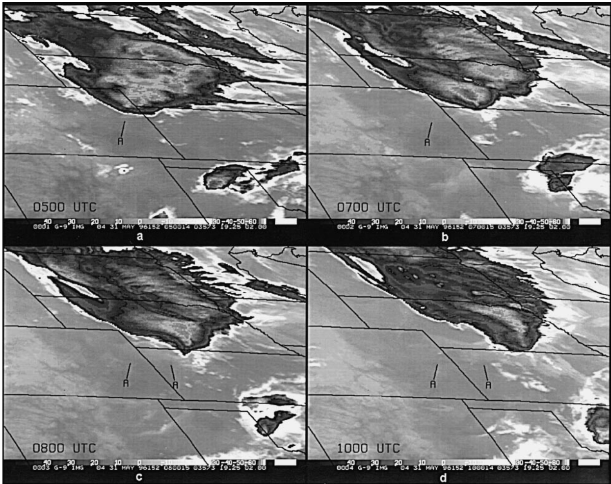
FIG. 1. The 10.7- \mu\text{m} imagery for the period 0500–1000 UTC 31 May 1996 showing a line of thunderstorms moving through Nebraska and South Dakota. The southern end of the complex is at the Nebraska–Kansas border at 0500 UTC. The leading edge of the rain-stabilized low-level thunderstorm outflow air at “A” (cf. to Fig. 2) is not clearly evident in these 10.7- \mu\text{m} satellite images because of a lack of thermal contrast between the clouds that formed along that boundary and the cool ground. The periods along the color bar at the bottom show the brightness temperatures in ^{\circ}\text{C} .
