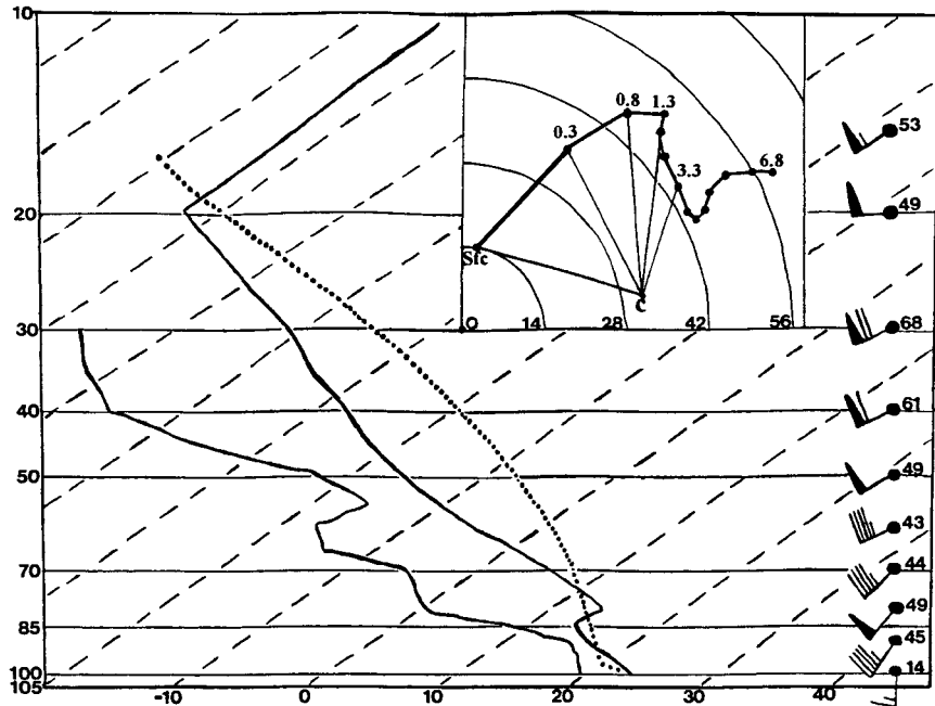
FIG. 2. The Paducah (PAH), KY, skew T sounding and hodograph (inset) at 1200 UTC 15 Apr. Winds in kt are shown at right. In the hodograph, numbers along the x-axis are wind speeds in kt, numbers along the hodograph curve represent km above the surface, and C is the default storm motion. Key thermodynamic parameters are given in the text.
