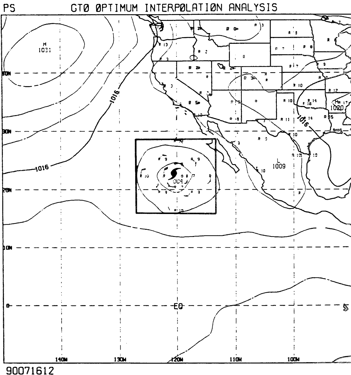
FIG. 4. Final optimum interpolation sea level pressure analysis with bogus wind reports (box A) for Hurricane Genevieve at 22°N, 120°W, 1200 UTC 16 July 1990.
