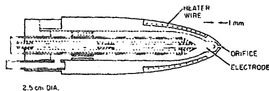
FIG. 1. Schematic diagram of the tip of the present model of the electrostatic disdrometer.
