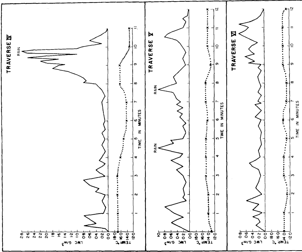
Fig. 3b. As in Fig. 3a except for traverses 4 to 6.
