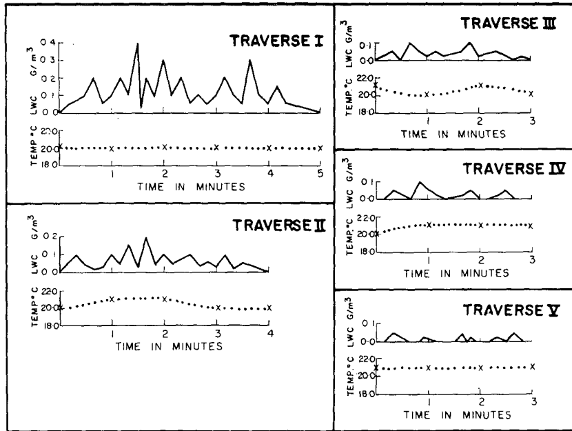
FIG. 1. Recordings of LWC and temperature in cloud complex A on 19 July 1973 (traverses 1 to 5).
