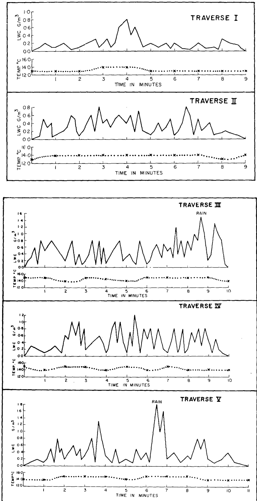
FIG. 4. Recordings of LWC and temperature in cloud complex on 13 August 1973.
