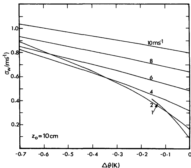
FIG. 1. Variation of \sigma_w with potential temperature difference between the 6.1 and 30.5 m levels for different values of surface wind speed u , for the unstable case.
