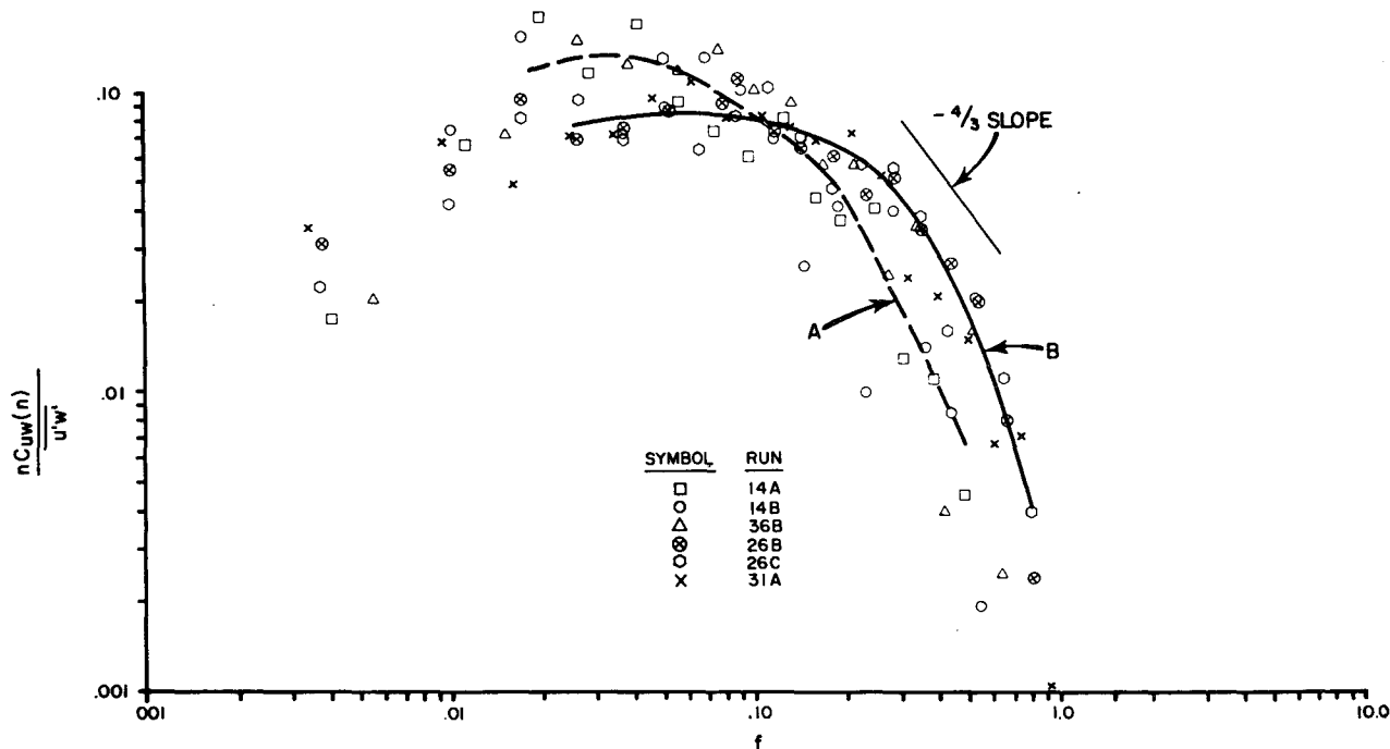
FIG. 5. Normalized logarithmic cospectra of vertical velocity and horizontal velocity fluctuations for conditions described in Fig. 1. Line with -4/3 slope in the inertial subrange is also shown.
