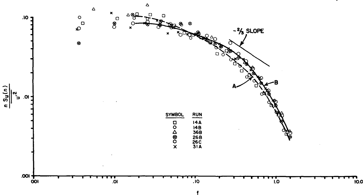
FIG. 2. As in Fig. 1 except for spectra of horizontal velocity fluctuations.
