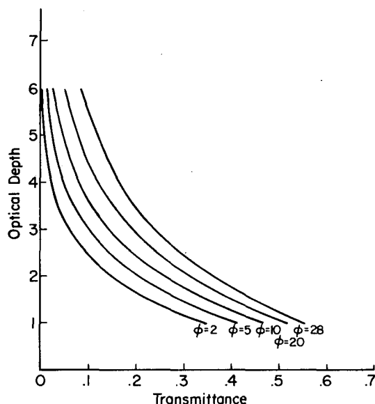
FIG. 1. Optical depth versus transmittance for fields of view \phi = 2, 5, 10, 20 and 28^\circ produced from the Monte Carlo model.
