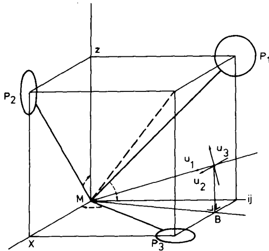
FIG. 1. Coordinate systems of the pressure anemometer ( x, y, z ) and the wind ( u_1, u_2, u_3 ). The u_1 component is along the mean wind, u_2 is perpendicular to u_1 and parallel to the xy -plane and u_3 is perpendicular to u_1 and u_2 . The dashed line is along the vertical, so the plane of P_1, P_2 and P_3 is horizontal. The ring with its center at P_1 is sensitive to the windcomponent in the x -direction only, those at P_2 and P_3 to the y - and z -component, respectively. The direction of the mean wind in this figure is very unusual (an elevation of about 60^\circ ) and was chosen only for graphical reasons.
