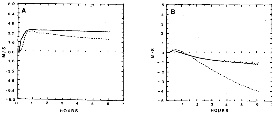
FIG. 10. (a) Times series of u -component at 2 meters (solid) and 50 meters (dashed) over the middle of the western sidewall ( x = 15, y = 23). (b) Times series of v -component at 2 meters (solid) and 50 meters (dashed) at the center of the valley ( x = 18, y = 23).
