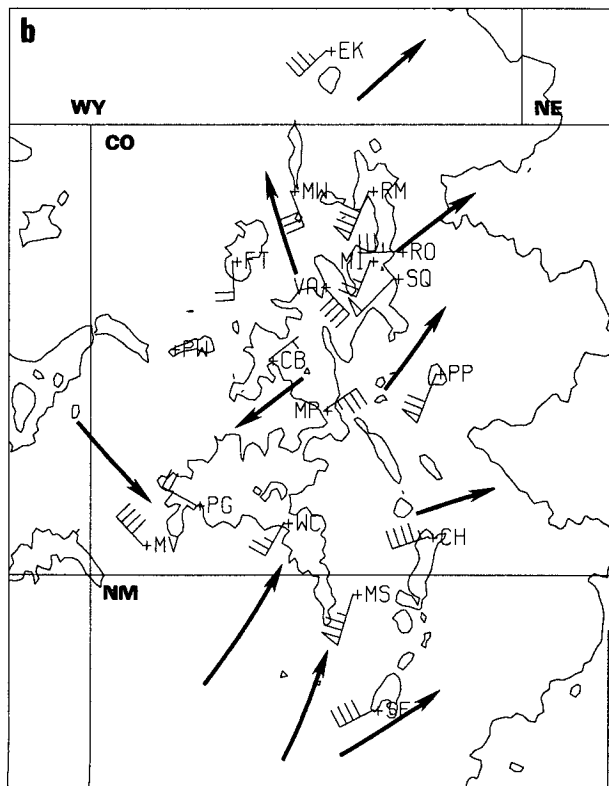
NOCTURNAL WIND DATA FOR 8/27/85
