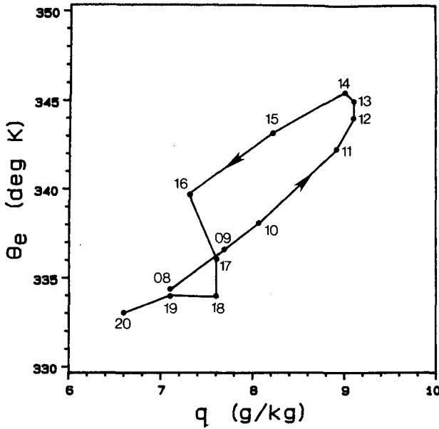
FIG. 10. Hourly averaged values at Mt. Werner of equivalent potential temperature versus mixing ratio for the labeled hours of 0800-2000 MST 13 August 1986.
