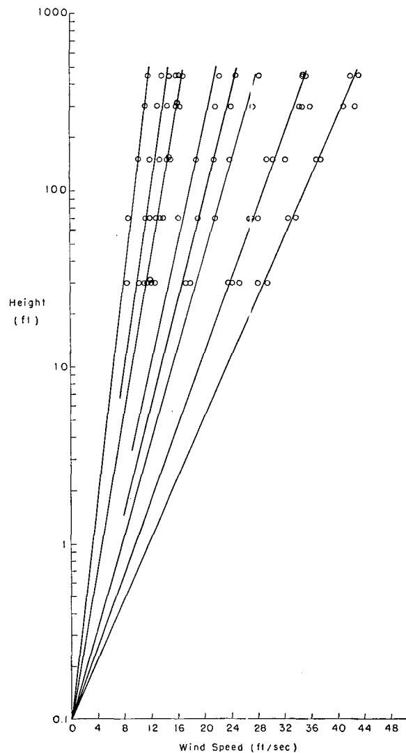
FIG. 1. Estimate of roughness length, z_0 , based on 14 near-adiabatic profiles.
