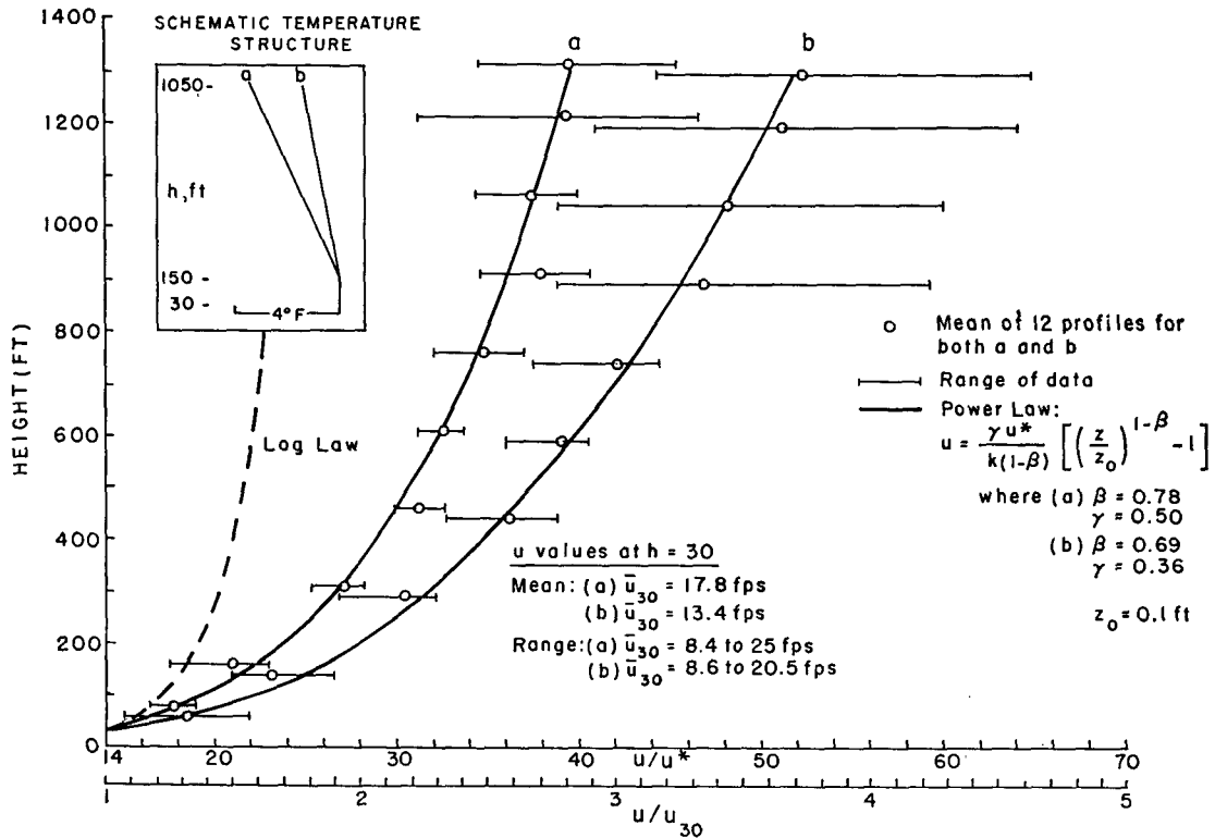
Fig. 6. Average wind profiles for a temperature stratification that is isothermal in the 30- to 150-ft layer and approximately \frac{1}{2} and \frac{1}{3} of the adiabatic rate in the 150- to 1050-ft layer.
