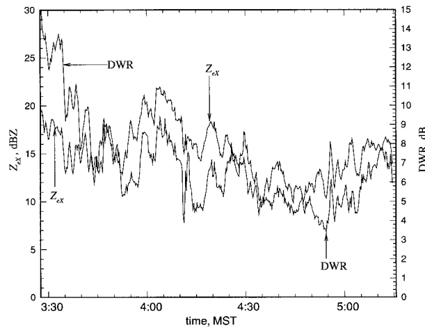
FIG. 8. Same as Fig. 5 but for the 14 March 1996 snowfall event.
