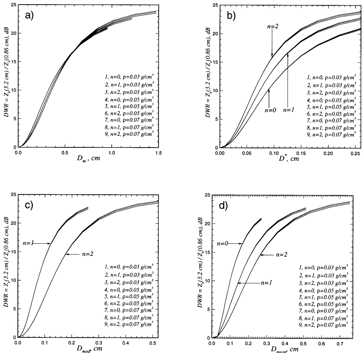
FIG. 2. Dual-wavelength ratio as a function of (a) snowflake median size D_m , (b) D^* , (c) modal size D_{mod} , and (d) mean size D_{mean} for spherical particles of different densities \rho and orders of the gamma-function size distributions ( n ).
