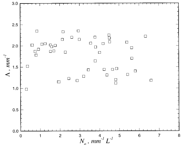
FIG. 1. Relation between parameters N_o and \Lambda in snowflake-size spectra.
