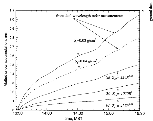
FIG. 6. Melted snow accumulation for the 25 January 1996 snowfall event from dual-wavelength radar measurements and from different existing single-parameter Z_{ex} - R relationships: (a) Boucher and Wieler (1985), (b) Puhakka (1975), and (c) Fujiyoshi et al. (1990).
