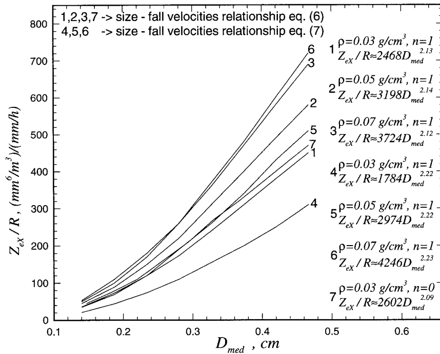
FIG. 3. The Z_e - R - D_m relationships at X band for different snowflake densities, fall velocity-size relationships, and orders of the gamma size distributions.
