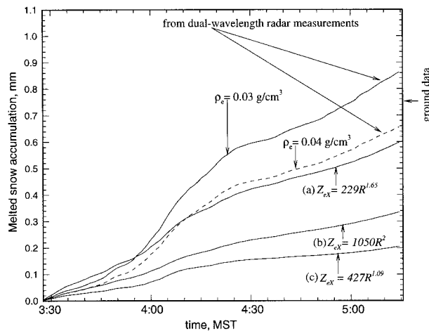
FIG. 9. Same as Fig. 6 but for the 14 March 1996 snowfall event.
