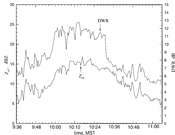
FIG. 10. Same as Fig. 5 but for the 26 February 1996 snowfall event.
