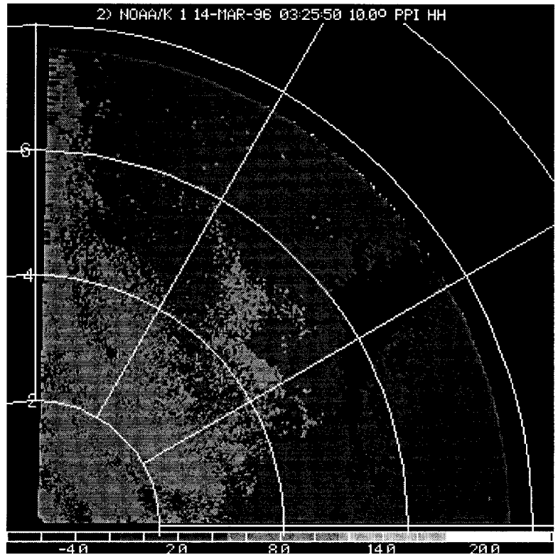
FIG. 7. Same as Fig. 4 but for the 14 March 1996 snowfall event.
