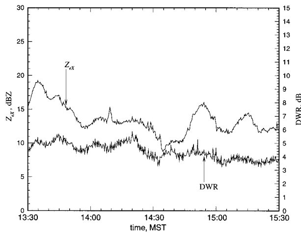
FIG. 5. Time series of the X-band reflectivity Z_{ex} and the dual-wavelength ratio DWR during the 25 January 1996 snowfall event.
