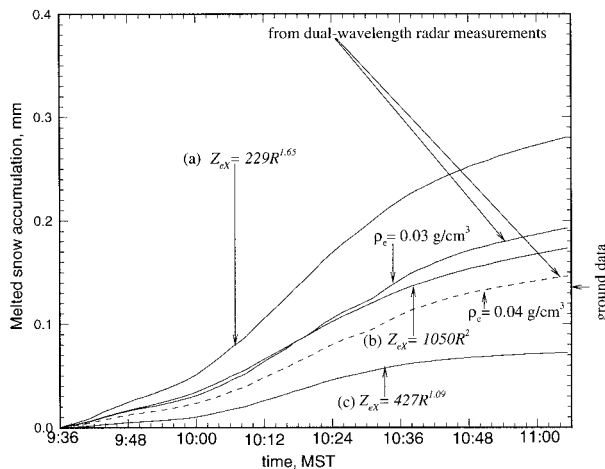
FIG. 11. Same as Fig. 6 but for the 26 February 1996 snowfall event.
