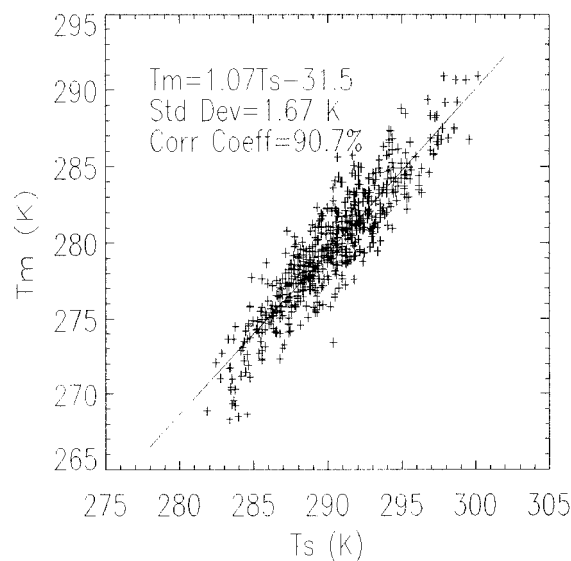
FIG. 1. Weighted mean temperature ( T_m ) vs surface temperature ( T_s ) at the Taipei site each Mar from 1988 to 1997.
