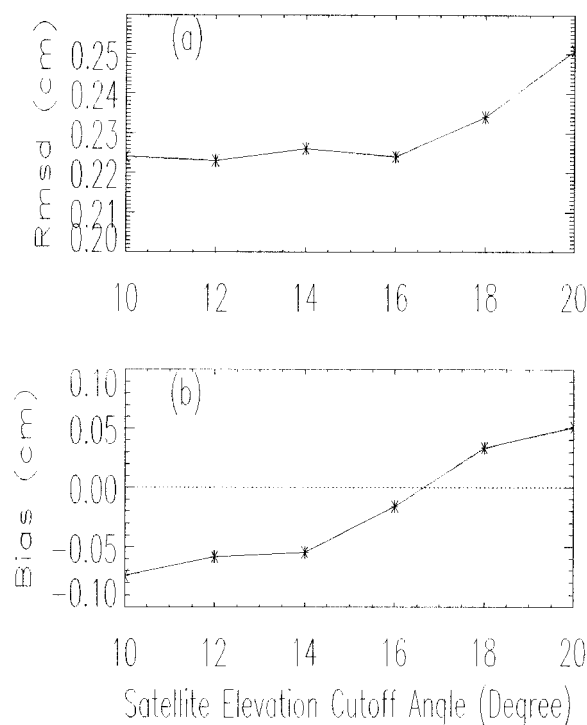
FIG. 10. (a) Rms difference and (b) bias in PW between GPS and WVR observations for six satellite elevation cutoff angles between 10^\circ and 20^\circ in 2^\circ increments for the Taipei-Tsukuba baseline case.
