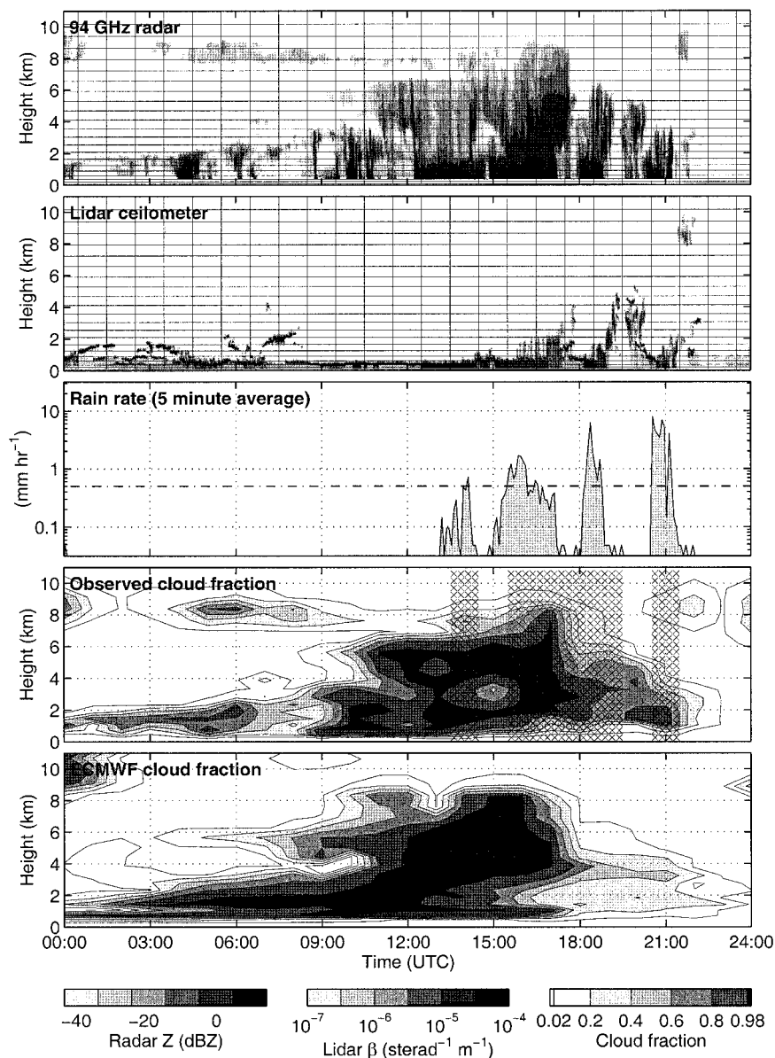
FIG. 2. An example of the retrieval of cloud fraction from radar and lidar data on 25 Dec 1998. Overlaid on the raw observations in the top two panels are the model grid boxes, and rain rate is shown in the third panel. The fourth panel depicts the cloud fraction retrieved from these observations, and the fifth shows the corresponding values held in the ECMWF model. The crosses on the observed cloud fraction field show periods when the comparison with the model was not performed because the rain rate at the surface exceeded 0.5 \text{ mm h}^{-1} at some time during the hour.
