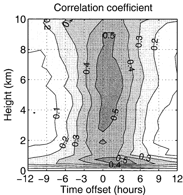
FIG. 11. The correlation coefficient between the observations and the model as a function of height and lag time, where a positive lag indicates a tendency for the model to simulate features before they were observed.
