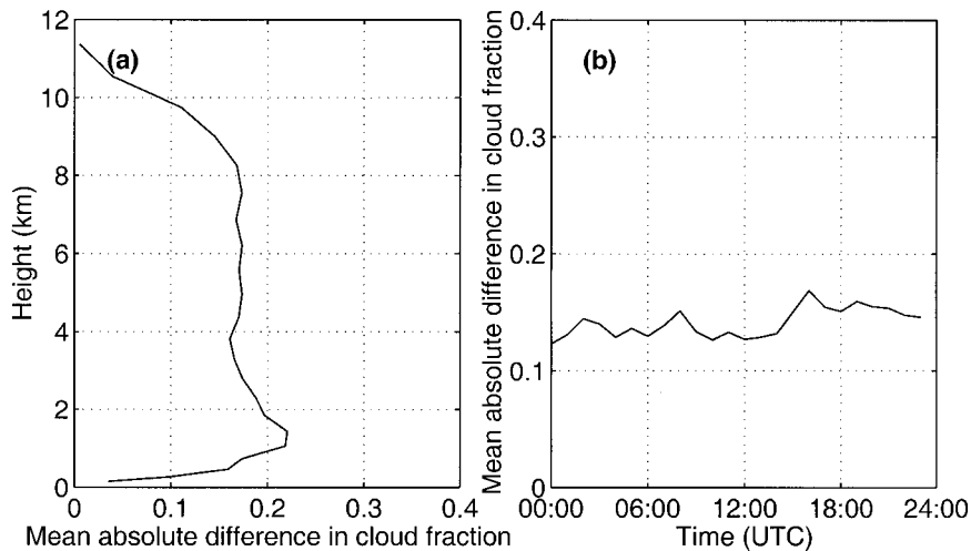
FIG. 10. Mean absolute difference in cloud fraction between the observations and ECMWF1 as a function of (a) height and (b) time of day.
