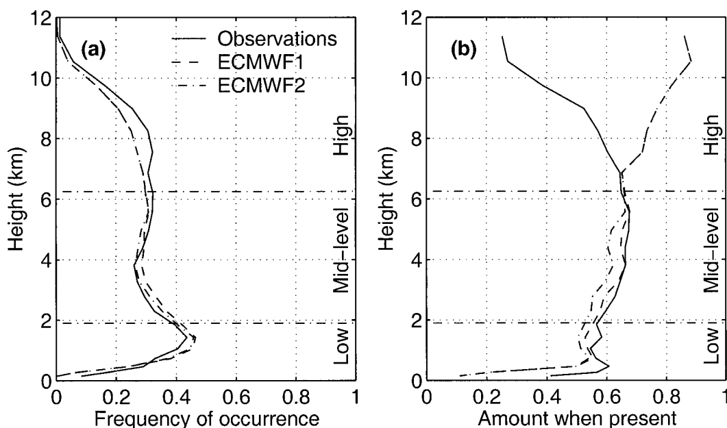
FIG. 9. The frequency of cloud occurrence and the mean amount when present for the observations and the two modified model fields that were used in Fig. 8.
