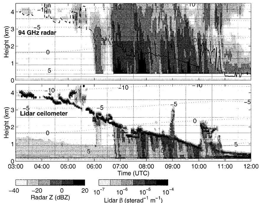
FIG. 1. Radar and lidar observations of light precipitation on 27 Nov 1998. Superimposed on the radar image is the position of cloud base according to the lidar, although above the melting layer it is not used in the retrieval of cloud fraction and is shown as a dashed line. The dotted contours depict the temperature in degrees Celsius according to the model.
