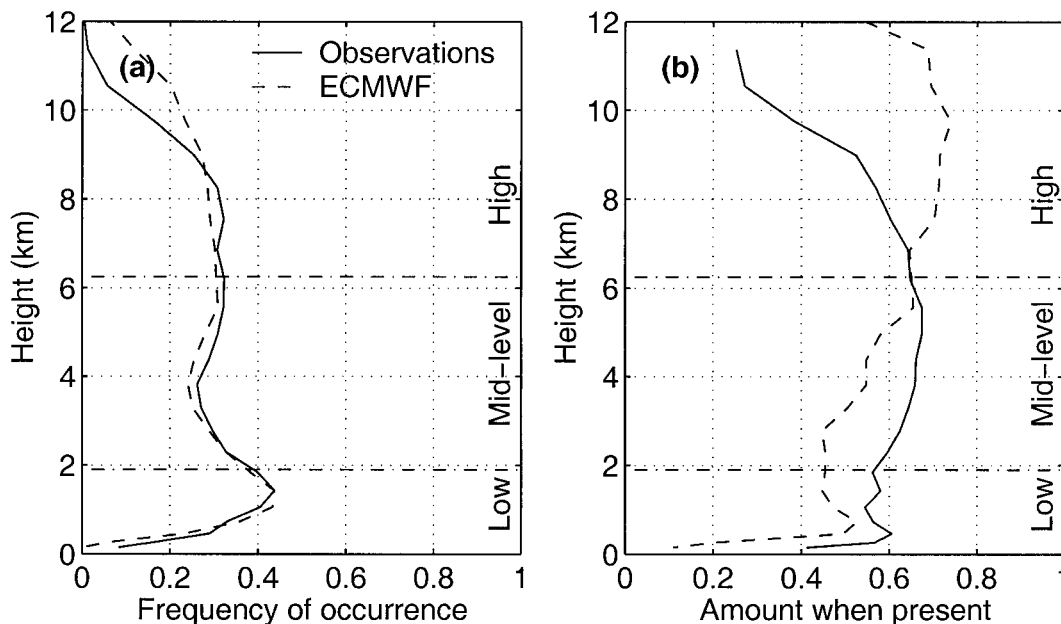
FIG. 5. Mean cloud fraction split into (a) the frequency that the gridbox-mean cloud fraction was greater than 0.05 and (b) the mean cloud amount when greater than 0.05.
