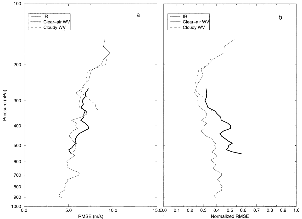
FIG. 1. (a) Rmse ( \text{m s}^{-1} ) between GOES winds and collocated raobs at individual height assignment level. (b) As in (a), but for normalized rmse.
