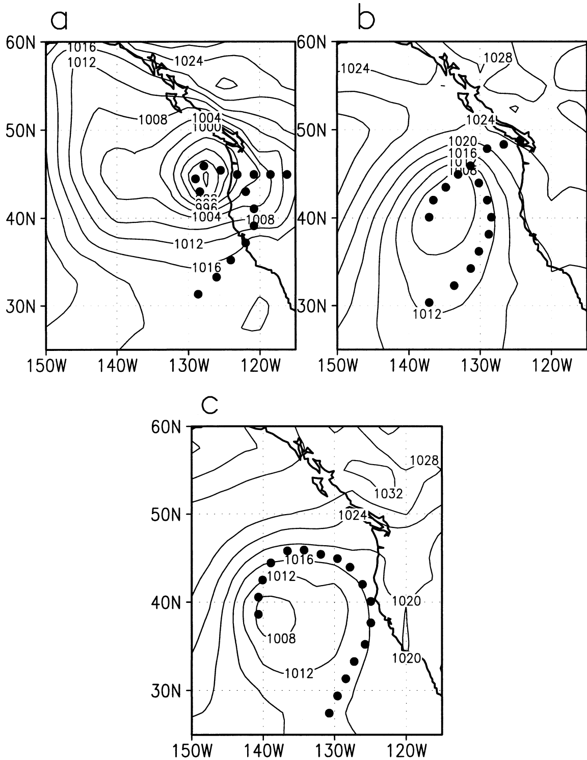
FIG. 9. ECMWF model analyses of MSLP (hPa) at (a) 1200 UTC 16 Jan, (b) 0000 UTC 18 Jan, and (c) 0000 UTC 19 Jan 2000. Dotted lines indicate frontal positions.
