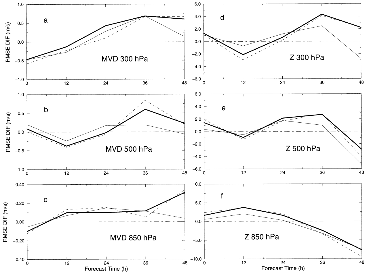
FIG. 12. Improvement over control run of SNGL (thin solid line), MULT (dashed line), and SLCT (thick solid line), of mean vector difference ( \text{m s}^{-1} ) and heights (m) at (a), (d) 300, (b), (e) 500, and (c), (f) 850 hPa. Values consist of rmse between verification data and CNTL minus rmse between verification data and SNGL, MULT, or SLCT. Positive values indicate an improvement (as compared with CNTL); negative values indicate a degradation (as compared with CNTL). Horizontal dash-dot line indicates value of zero.
