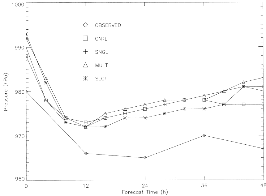
FIG. 11. Minimum MSLP (hPa) of storm during forecast within each simulation.
