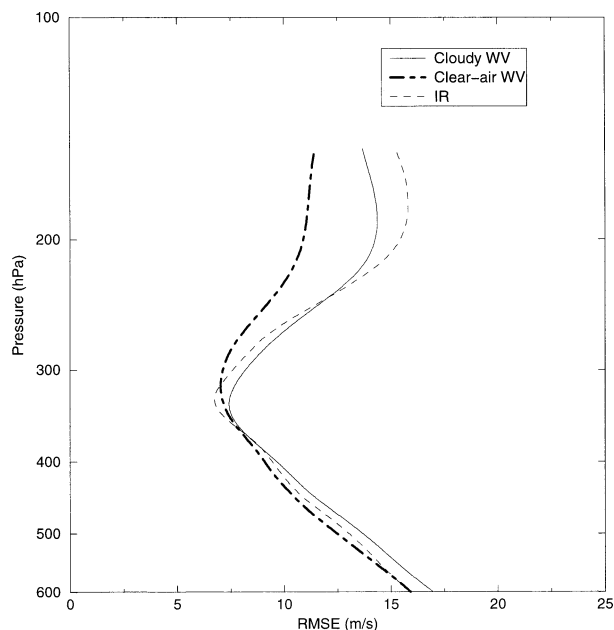
FIG. 2. Rmse ( \text{m s}^{-1} ) between 300-hPa GOES winds and entire profile of collocated raobs.
