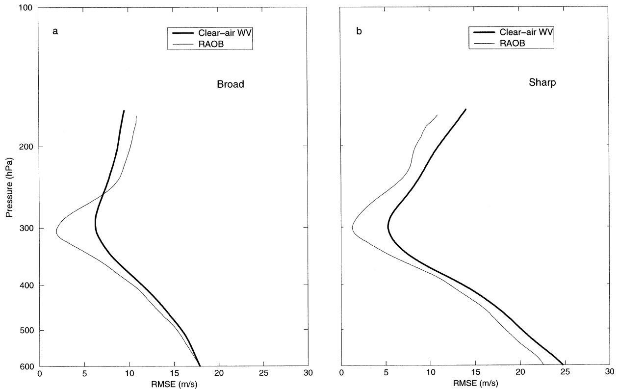
FIG. 5. (a) Broad CA WV profile (Fig. 3a) for 300-hPa height assignments along with corresponding NC profiles ( \text{m s}^{-1} ) as described in the text. (b) As in (a), but for sharp category.
