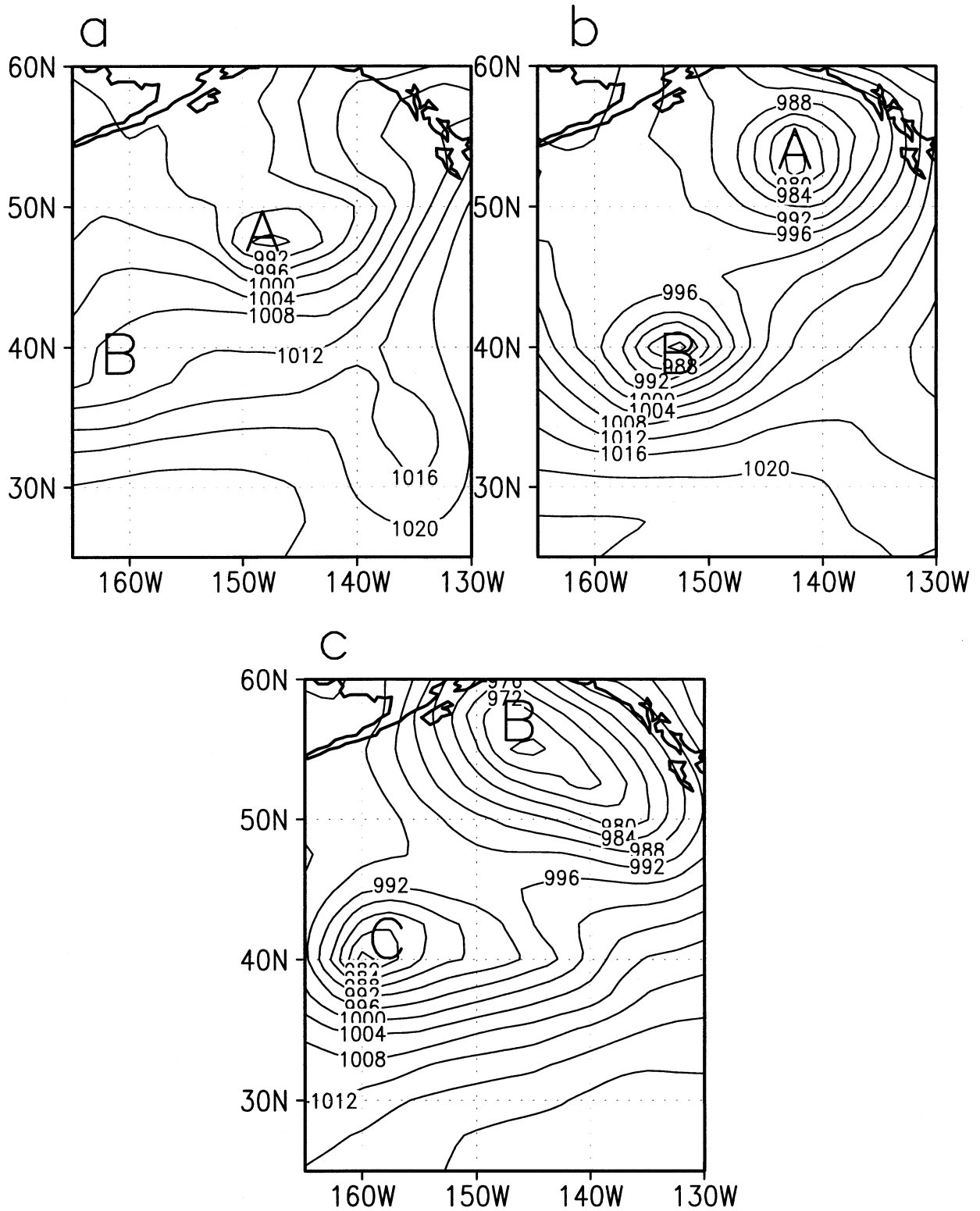
FIG. 7. ECMWF model analyses of MSLP (hPa) at (a) 1200 UTC 28 Jan, (b) 0000 UTC 29 Jan, and (c) 1200 UTC 31 Jan 2000. Points A, B, and C represent series of cyclones that were present during the simulation.
