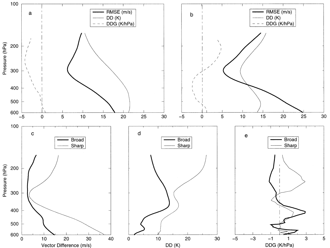
FIG. 3. (a) Rmse ( \text{m s}^{-1} ), mean DD (K), and mean DDE ( 5 \times \text{K hPa}^{-1} ) within the broad category of CA WV winds at a height assignment of 300 hPa. (b) As in (a), but for the sharp category. Representative profiles of the (c) vector difference ( \text{m s}^{-1} ), (d) DD (K), and (e) DDG ( \text{K hPa}^{-1} ). Vertical dash-dot line in (a), (b), and (e) indicates a value of zero.
