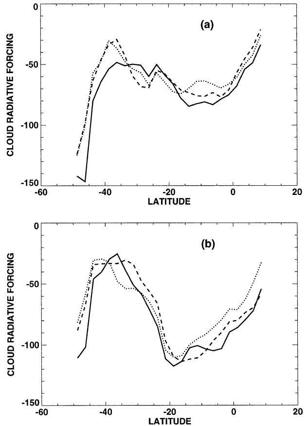
FIG. 3. (a) SRB monthly mean cloud radiative forcing in Jan 1986 (solid), 1987 (dotted), and 1988 (dashed); (b) model-simulated data.
