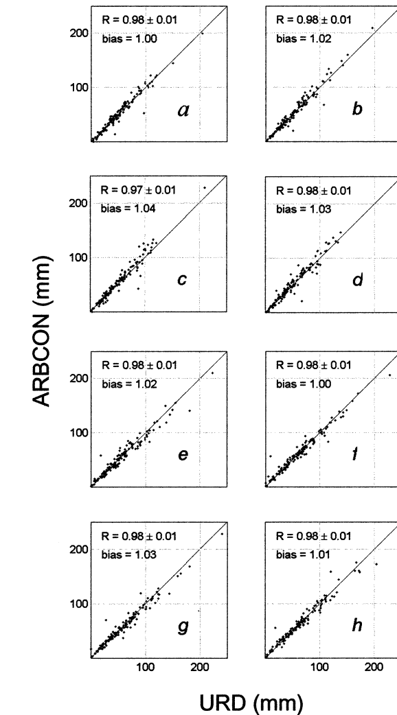
FIG. 3. Comparison of the monthly, 1.25^\circ \times 1.25^\circ grids, rainfall estimates obtained from ARBICON and URD for the two validation sites in North Dakota. The identification letters represent the subboxes shown in Fig. 1.
