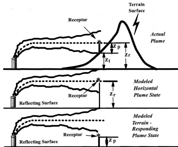
FIG. 1. AERMOD two-state approach. The total concentration predicted by AERMOD is the weighted sum of the two extreme possible plume states: the horizontal plume state and the terrain-following state.
