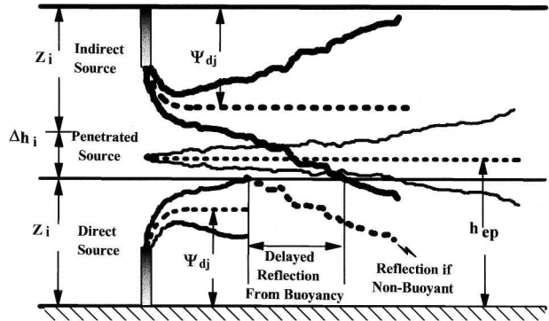
FIG. 3. AERMOD’s three-plume treatment of the CBL.
