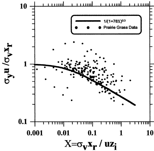
FIG. 2. Lateral spread ( \sigma_y ) as a function of nondimensional distance ( X ). The data are taken from the Prairie Grass Experiment (Barad 1958).
