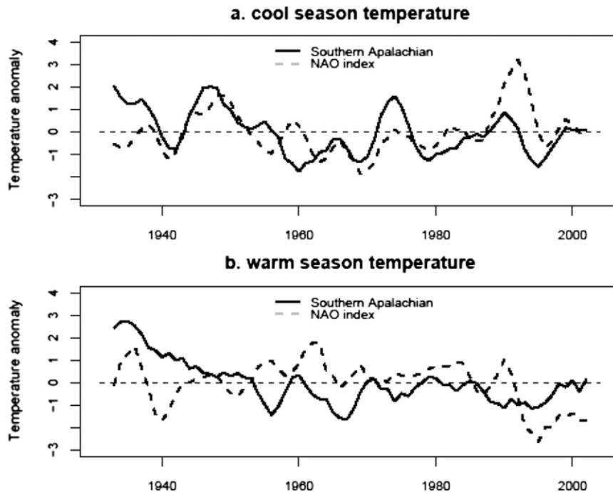
FIG. 2. Standardized anomalies for southern Appalachian (solid line) and NAO index (dashed line) for the years 1931–2004 by (top) cool (November–April) and (bottom) warm (May–October) seasons. The climate anomalies are the difference between the 5-yr weighted means and the weighted mean for the base period 1951–80. The anomalies were standardized to a normal distribution with mean = 0 and standard deviation = 1 to illustrate disparate trends at the same scale.
