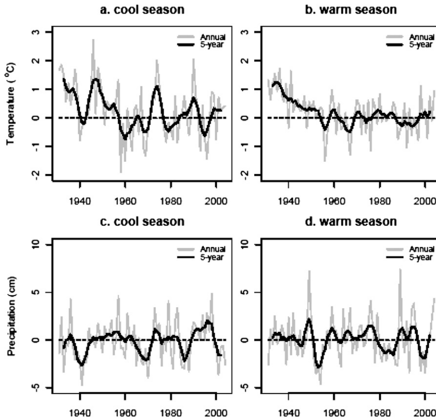
FIG. 1. Southern Appalachian region (top) temperature and (bottom) precipitation trends by cool (left) (November–April) and warm (right) (May–October) seasons. The trends are represented by annual means (gray line) and center-weighted 5-yr means (black line) of southern Appalachian mean temperature and precipitation anomalies (1931–2004). The climate anomalies are the difference between the yearly means and the mean for the base period 1951–80.
