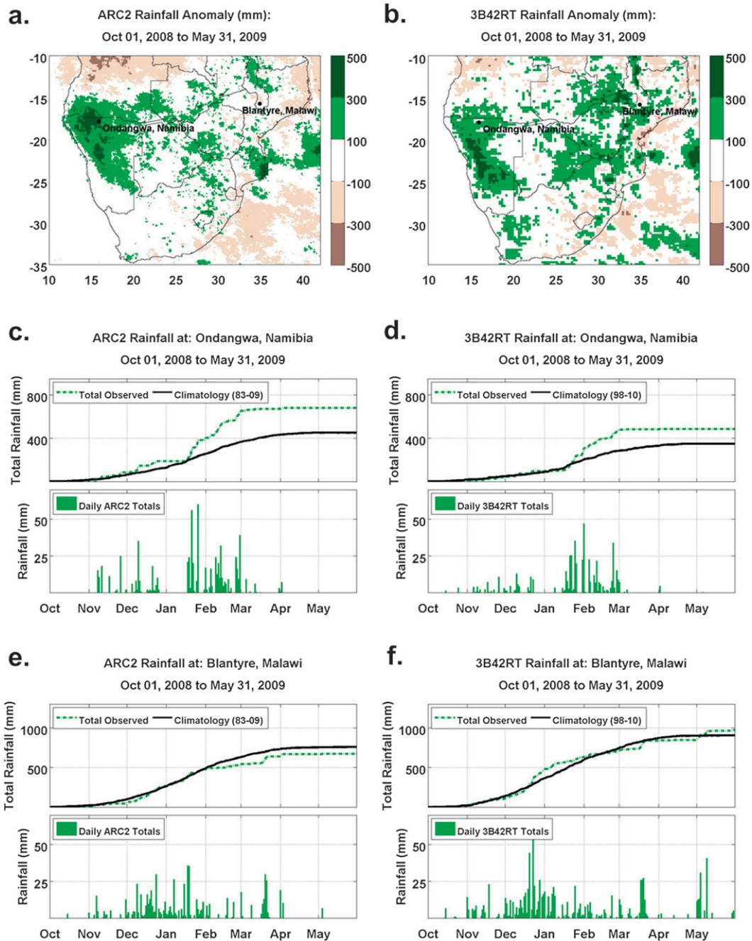
FIG. 11. Map of (a) ARC2 rainfall anomaly (mm), (b) 3B42RT total rainfall anomaly (mm), and observed and accumulative (c) ARC2, as well as (d) 3B42RT rainfall time series from Ondangwa, and (e) ARC2 and (f) 3B42RT rainfall time series of Blantyre, for the southern Africa rainy season (1 Oct 2008–31 May 2009).
