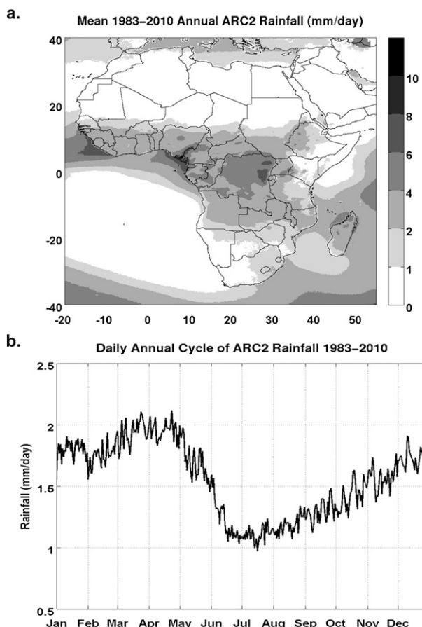
FIG. 1. (a) Spatial mean of annual ARC2 rainfall ( \text{mm day}^{-1} ) at 0.1^\circ resolution over Africa from 1983 to 2010 and (b) daily annual cycle of ARC2 rainfall ( \text{mm day}^{-1} ) over the African domain ( 40^\circ\text{S} – 40^\circ\text{N} and 20^\circ\text{W} – 55^\circ\text{E} ) from 1983 to 2010.
