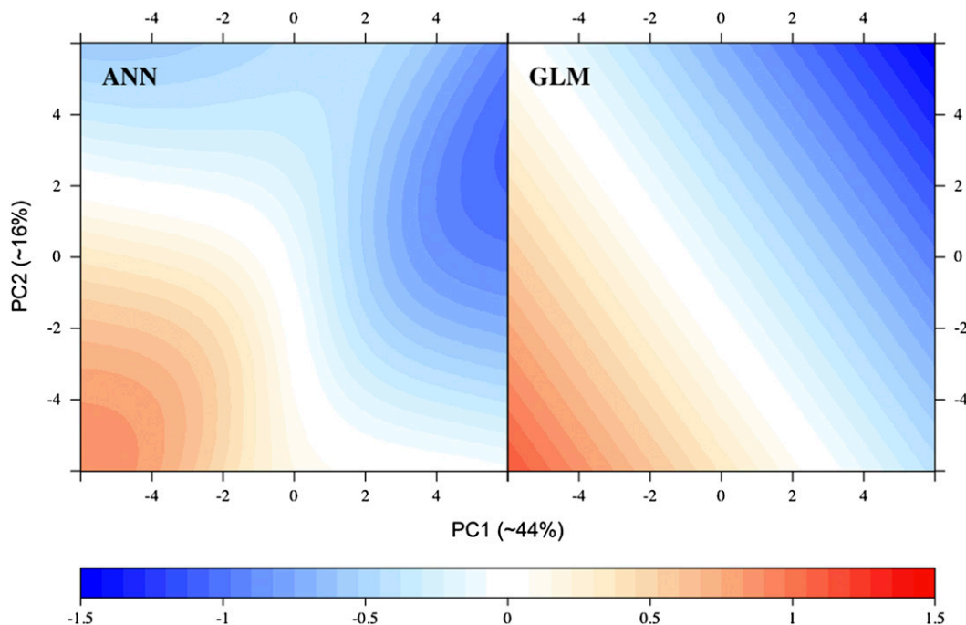
FIG. 12. Two-dimensional partial dependence of the Sahelian rainfall anomaly as a function of changes in both PC1 and PC2. ANN captures the nonlinear interactions among variables, while GLM approximates all relations in linear forms.
