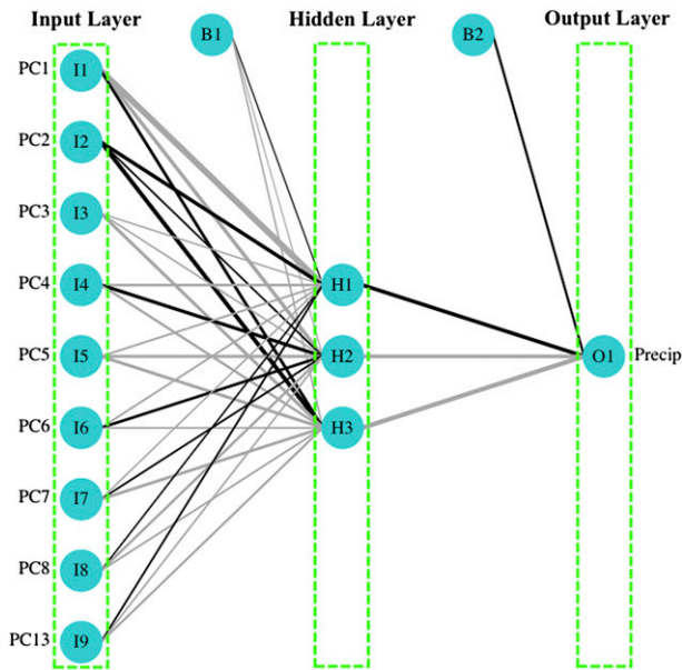
FIG. 4. Schematic diagram for the ANN in the final ANN model. It is a feed-forward single-layer network with three units in the hidden layer. The connections between nodes are shown in black (gray) lines for positive (negative) weights. Line thickness is proportional to relative weight. The nine nodes in the input layer units (labeled as I1–I9) represent the nine PCs used as covariates in the model, and the response variable is shown in the output layer unit (labeled as O1). The hidden layer units are labeled as H1–H3 (three units), which were specified using cross-validated tuning of the hidden layer size. B1 and B2 are bias layers that apply constant values to the nodes, similar to intercept terms in a regression models.
