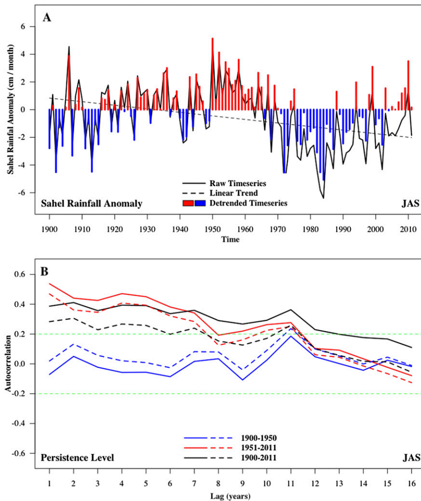
FIG. 1. Sahelian rainfall and its persistence. (a) Summer (JAS) time series for the period 1900–2011 and (b) autocorrelation vs lag (yr) of raw (solid lines) and detrended (dashed lines) time series over different time periods: 1900–50, 1951–2011, and the entire 1900–2011 record.
