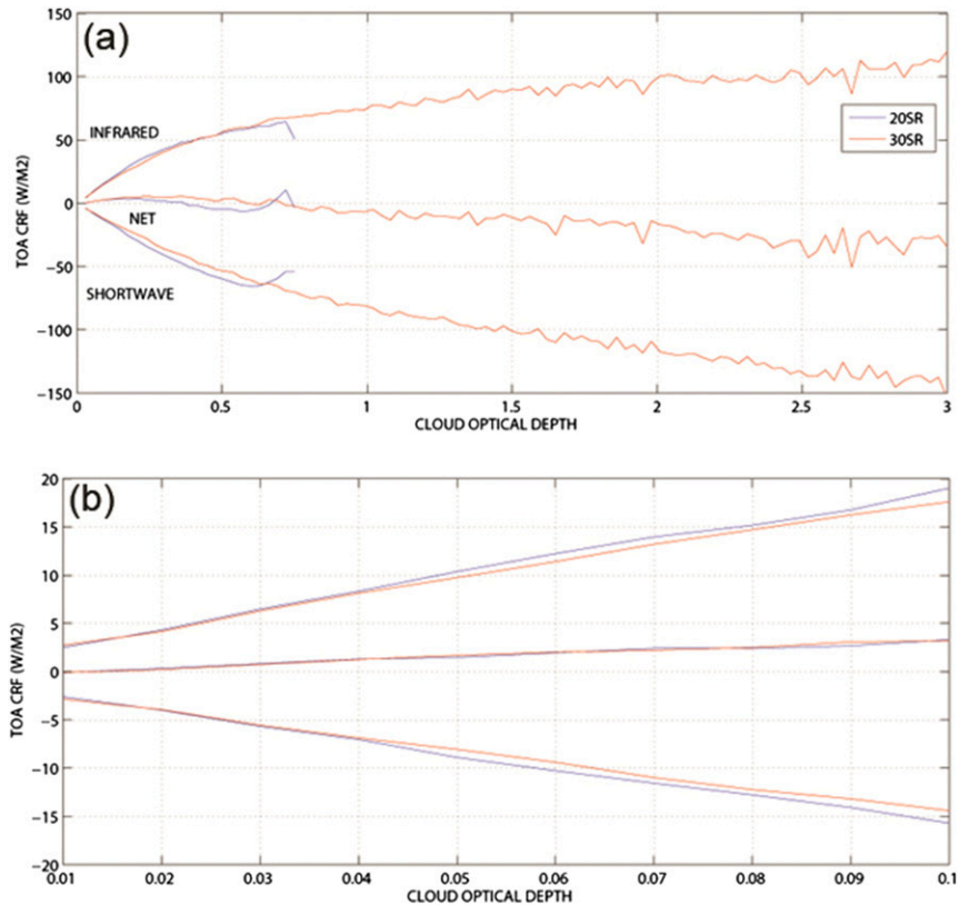
FIG. 2. For the 2012 daytime GSFC cirrus cloud subset, average TOA IR, SW, and net CRF for CODs (a) between 0.0 and 3.0 and (b) between 0.01 and 0.10, for the 20-sr (blue) and 30-sr (red) S -value solutions.
