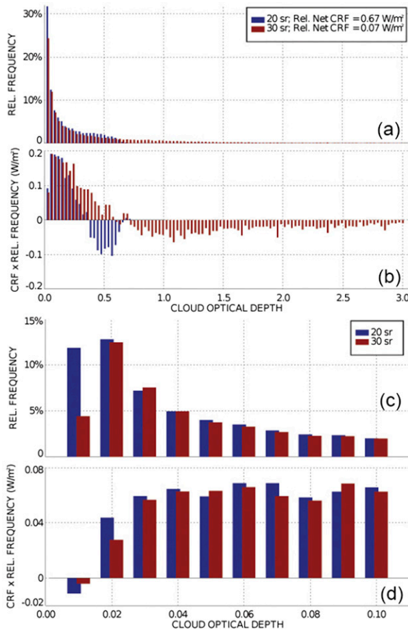
FIG. 3. For the 2012 daytime GSFC cirrus cloud subset, (a) relative frequency of cloud occurrence vs COD and (b) average net TOA CRF from Fig. 2a normalized by relative frequency in (a), both in 0.03 COD intervals between 0.0 and 3.0 for the 20-sr (blue) and 30-sr (red) S -value solutions. (c), (d) As in (a) and (b), but in 0.01 COD intervals between 0.0 and 0.1.
