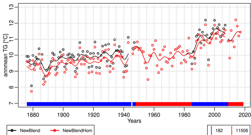
FIG. 8. Annual mean of the blended TG series of Rheinstetten. The color code is as in Fig. 5. The red bar indicates data from Rheinstetten (11 506); the blue bar indicates data from Karlsruhe (182).
