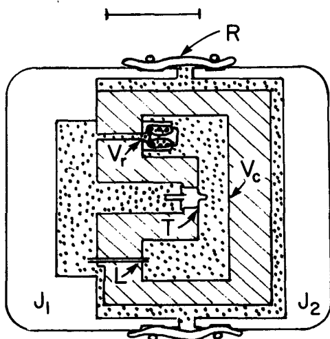
FIG. 4. Construction of the differential pressure gauge. The symbols are repeated from Fig. 2a. J_1 and J_2 are two parts of an acrylic plastic jacket that provides mechanical and thermal insulation. They are held together by the flexible rubber band R . Their relative motion, and motion of the rubber, admits ocean pressure to the interior of the gauge. V_1 is one of the two over-pressure relief valves. The aluminum wall of the reference chamber V_c is cross-hatched and the silicone oil is stippled. The differential transducer T is located at the center of volume of the reference chamber. L is the capillary leak. The scale bar is 50 mm in length.
