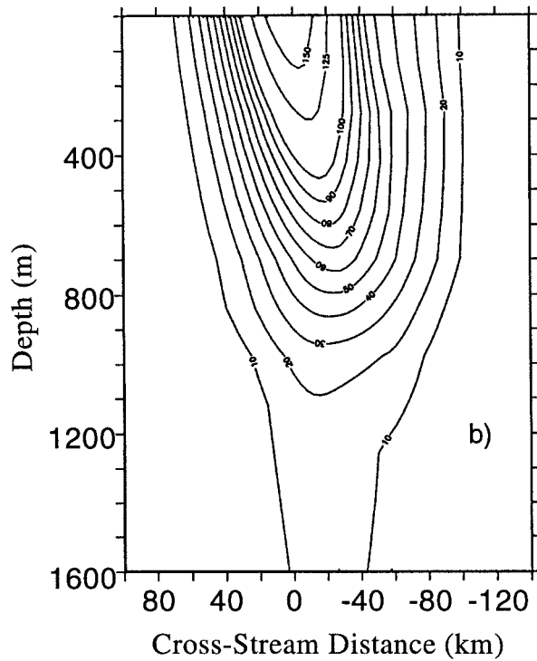
FIG. 5. Gulf Stream velocity sections (a) from Pegasus average synoptic profile and (b) from multiscale feature model.
