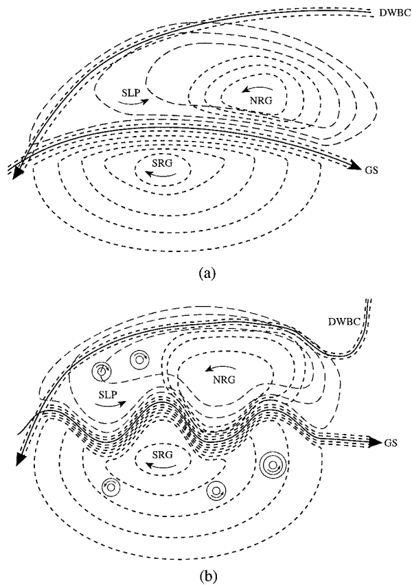
FIG. 9. Schematics of the recirculation gyres within the Gulf Stream system: (a) The mean state and (b) typical synoptic state with deformed ellipses.
