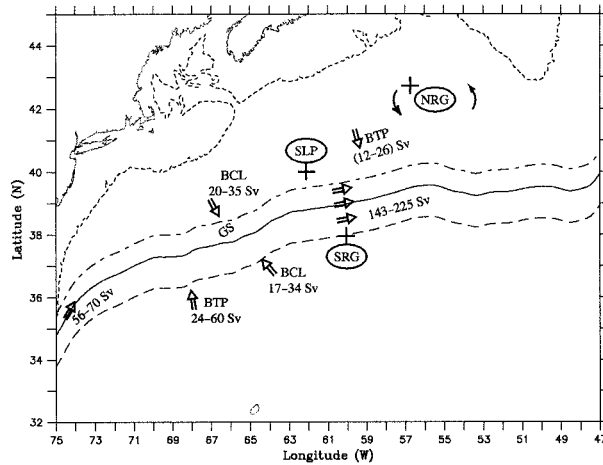
FIG. 11. The transport cartoon as derived from the circulation model analysis. The centers of the SBS gyres are marked as a plus sign. The ranges of transport influx from various gyres into the GS are depicted as part barotropic and part baroclinic.
