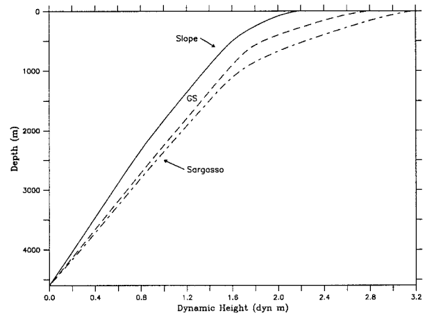
FIG. 4. Averaged profiles of dynamic height anomaly for the slope and Sargasso regions obtained from Levitus climatology and analytical GS structure (derived from the Pegasus synoptic profiles).
