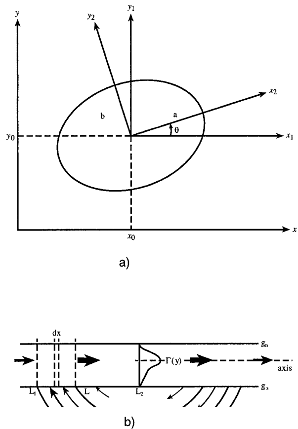
FIG. 10. (a) Schematic of an elliptic gyre. (b) A synoptic perspective of the kinematic synthesis.
