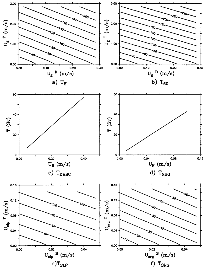
FIG. 12. Transport as a function of top and bottom velocities: (a) Gulf Stream at Cape Hatteras, (b) Gulf Stream at 60°, (c) DWBC, (d) NRG, (e) SLP, and (f) SRG.
