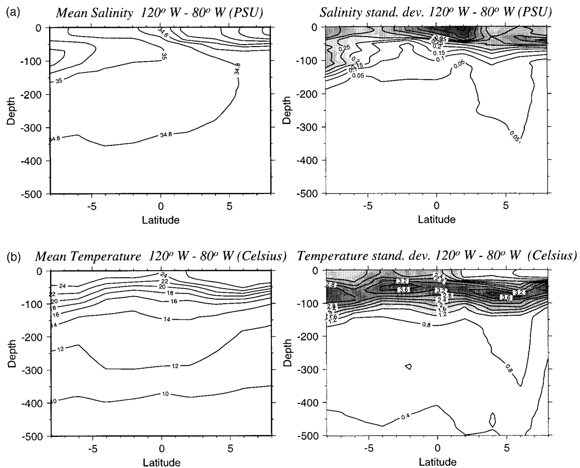
FIG. 4. (a) Salinity mean and standard deviation and (b) temperature. As in Fig. 2, but for the eastern Pacific (80°–120°W).
