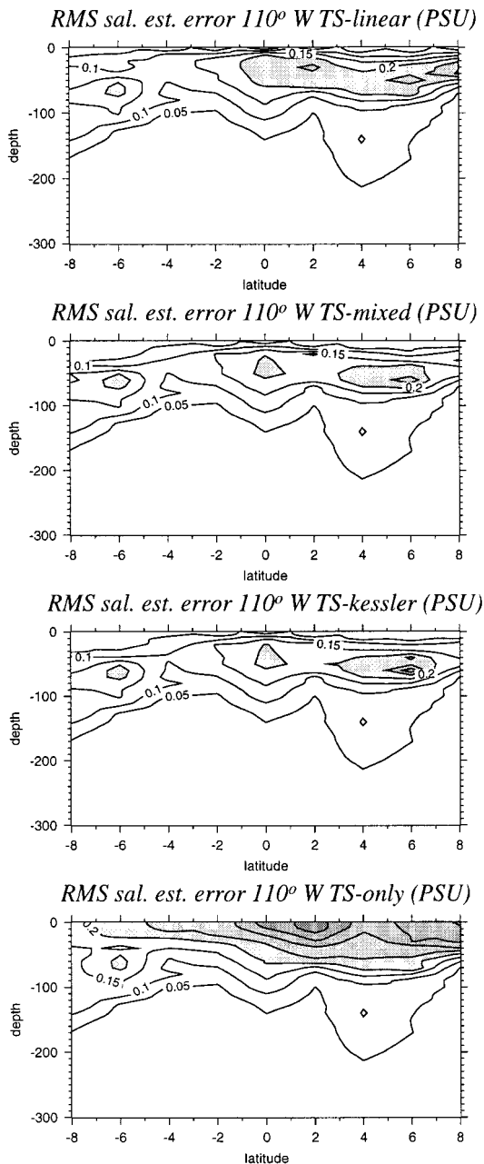
FIG. 8. Depth–latitude cross sections along 110^{\circ}\text{W} : rms difference between salinity as estimated by each of the four T–S estimation methods and observed salinity. As in Fig. 7.
