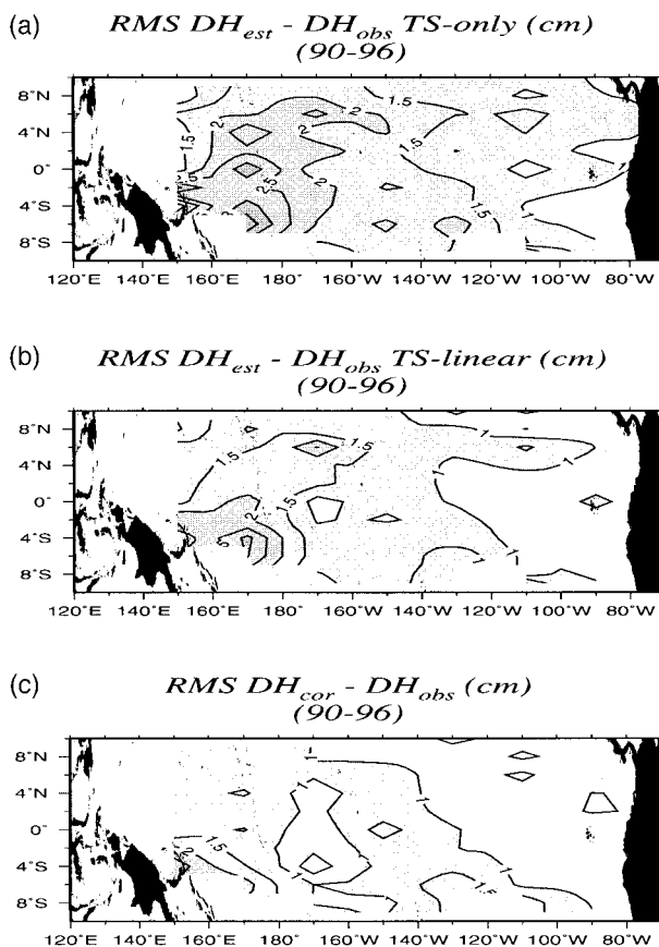
FIG. 11. (a) The rms of the dynamic height estimation error when salinity is estimated with the TS-only. (b) Same, but for TS-linear. (c) The rms dynamic height estimation error after EOF correction of the TS-linear salinity estimate. Analysis is based on CTD data from 1990–96.
