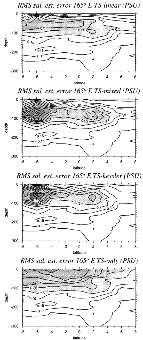
FIG. 7. Depth-latitude cross sections along 165°E: the rms difference between salinity as estimated by each of the four T-S estimation methods and observed salinity, applied on the CTDs for the period 1979–89. TS-linear: linear interpolation salinity from depth of isothermal layer to surface. TS-mixed: constant salinity from depth of isothermal layer to surface. TS-Kessler: linear interpolation T-S relation from depth isothermal layer to surface. TS-only: just the climatological relation. The rms values greater than 0.2 psu are shaded. Contour interval is 0.05 psu.
