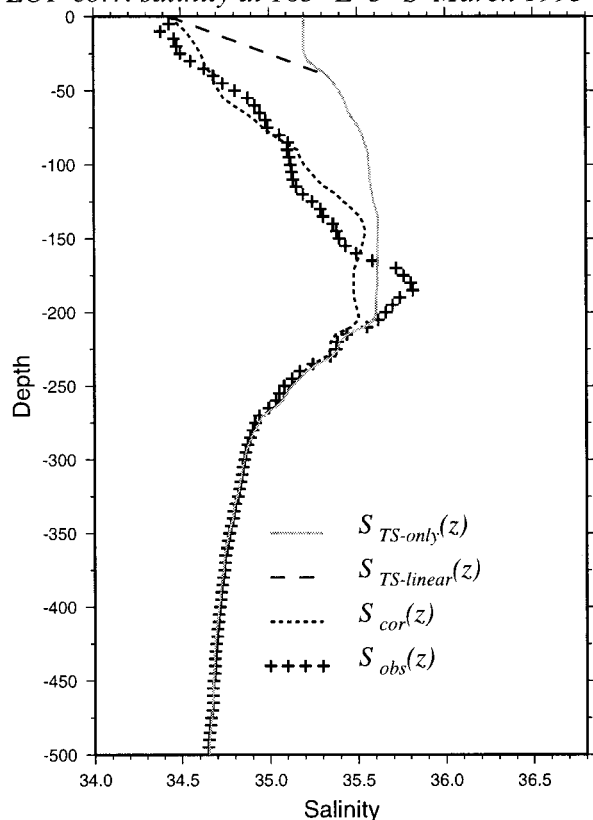
FIG. 10. Salinity correction with the use of dynamic height difference and the first EOF of the salinity estimation error using TS-linear. The method is demonstrated with the use of a CTD profile at 5°S, 165°E in Mar 1993. The profile for S_{est}(z) from TS-only is also shown for comparison.
