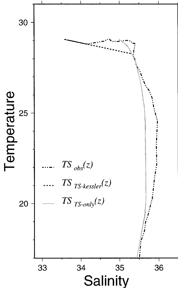
FIG. 6. Temperature vs salinity in a CTD profile in Jan 1989 at 6°S, 165°E. The TS-Kessler and TS-only salinity estimates are demonstrated with line types as in Fig. 5.
