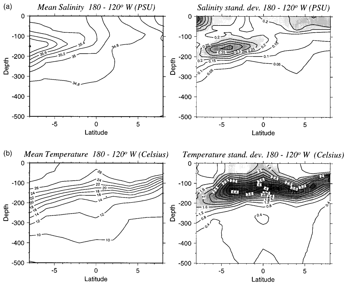
FIG. 3. (a) Mean and standard deviation salinity and (b) temperature. As in Fig. 2, but for the central Pacific (120°W–180°).
