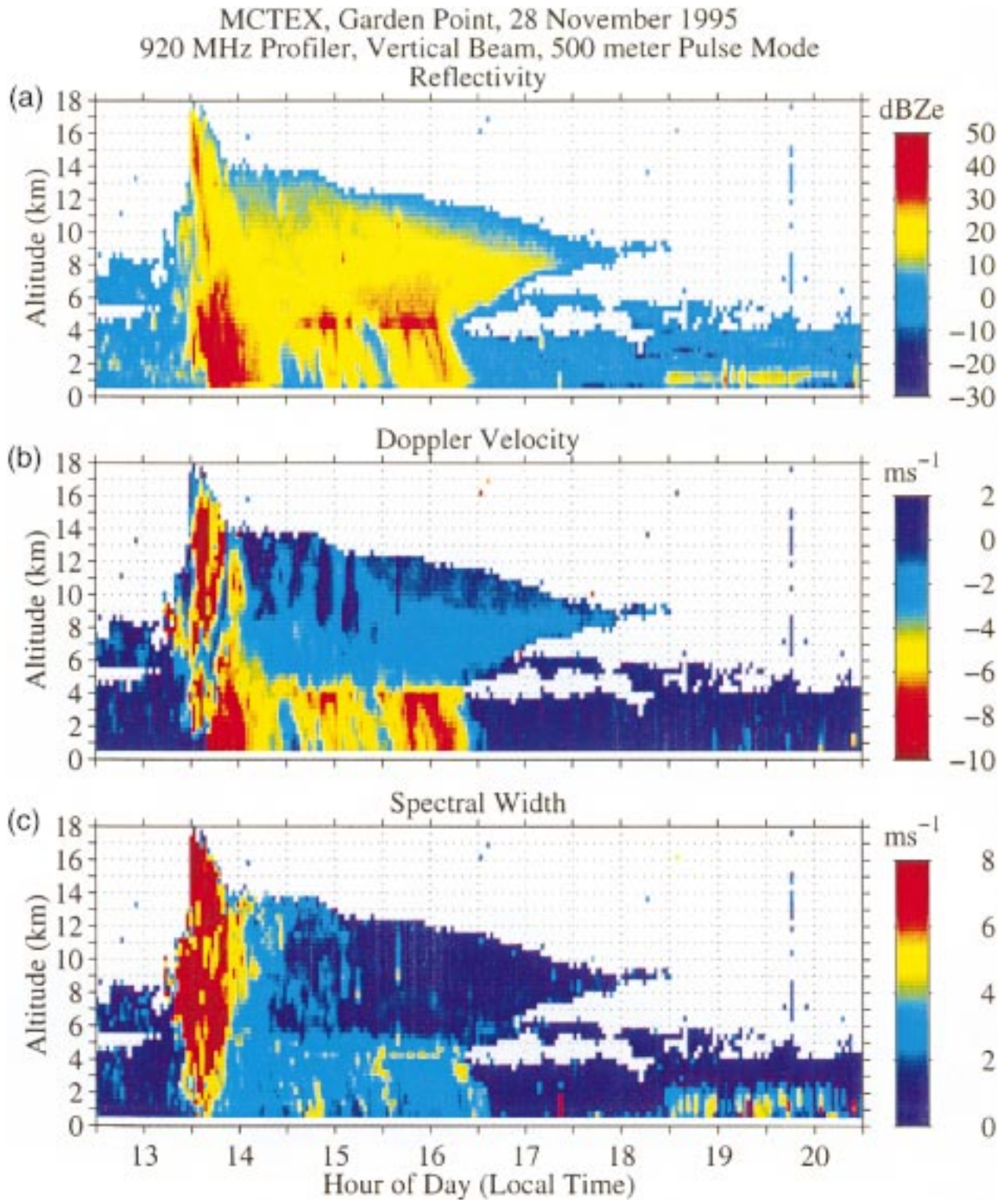
FIG. 6. Time–height sections of (a) equivalent reflectivity, (b) Doppler velocity, and (c) spectral width for observations made by the 920-MHz profiler at Garden Point on 28 November 1995.
