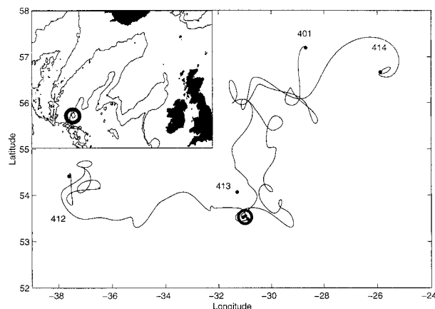
FIG. 4. Charts of the northeastern Atlantic Ocean. Labrador Sea water penetrates through Charlie Gibbs Fracture Zone into the Iceland Basin: 110 km east of this gap in the Mid-Atlantic Ridge we had installed our first float park (circle). The trajectories of four floats demonstrate the high amount of eddy noise and variability of the mean current in the intermediate water. To avoid unnecessary confusion the fourth trajectory (413), which resembles a random walk regime, was omitted in the figure. All surface locations are labeled by black dots. Before plotting, data were low-pass filtered (cut-off period 10 day) excluding small-scale tracking noise. For further details see Table 1.
