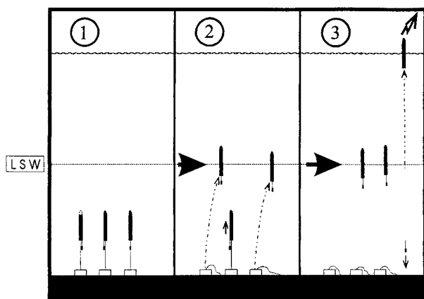
FIG. 1. (1) A float park consists of a number of temporarily moored RAFOS floats. (2) After a predetermined time individual floats depart from their anchors and ascend to their mission depths where they are subsequently advected horizontally. (3) At the end of their mission they drop a ballast weight, return to the sea surface, and transmit their stored data, i.e., typically the daily time-of-arrival signals from moored sound sources, and temperature and pressure data. The first float park was successfully tested east of Charlie Gibbs Fracture Zone (depth > 3500 m) in the Northeast Atlantic. Floats monitored the drift of Labrador Sea Water (LSW).
