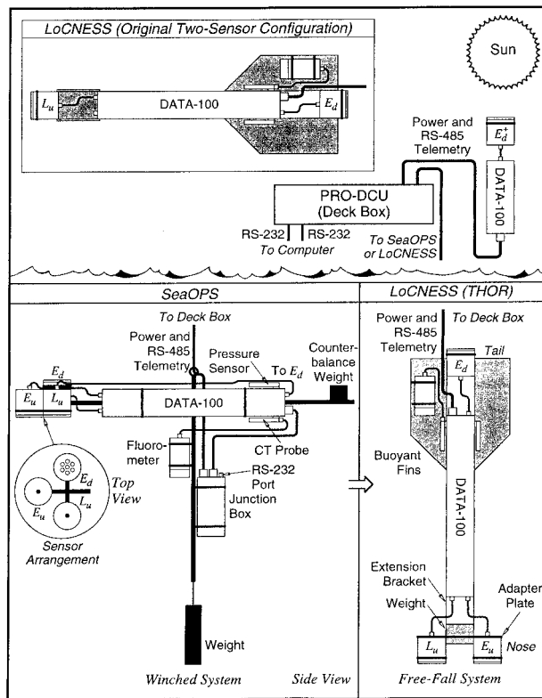
FIG. 2. A schematic showing the conversion of SeaOPS into LoCNES (top, inset panel) with the THOR configuration (right, bottom panel). The deck box provides the (computer controlled) DC power for all of the sensors and is designed to avoid instrument damage due to improper power-up sequences over varying cable lengths. The SeaOPS frame was modified before AMT-6, so three sensors could be clustered together (the third sensor connects to a third port on the DATA-100). LoCNES was modified at the same time, so two sensors could be mounted on the nose.
