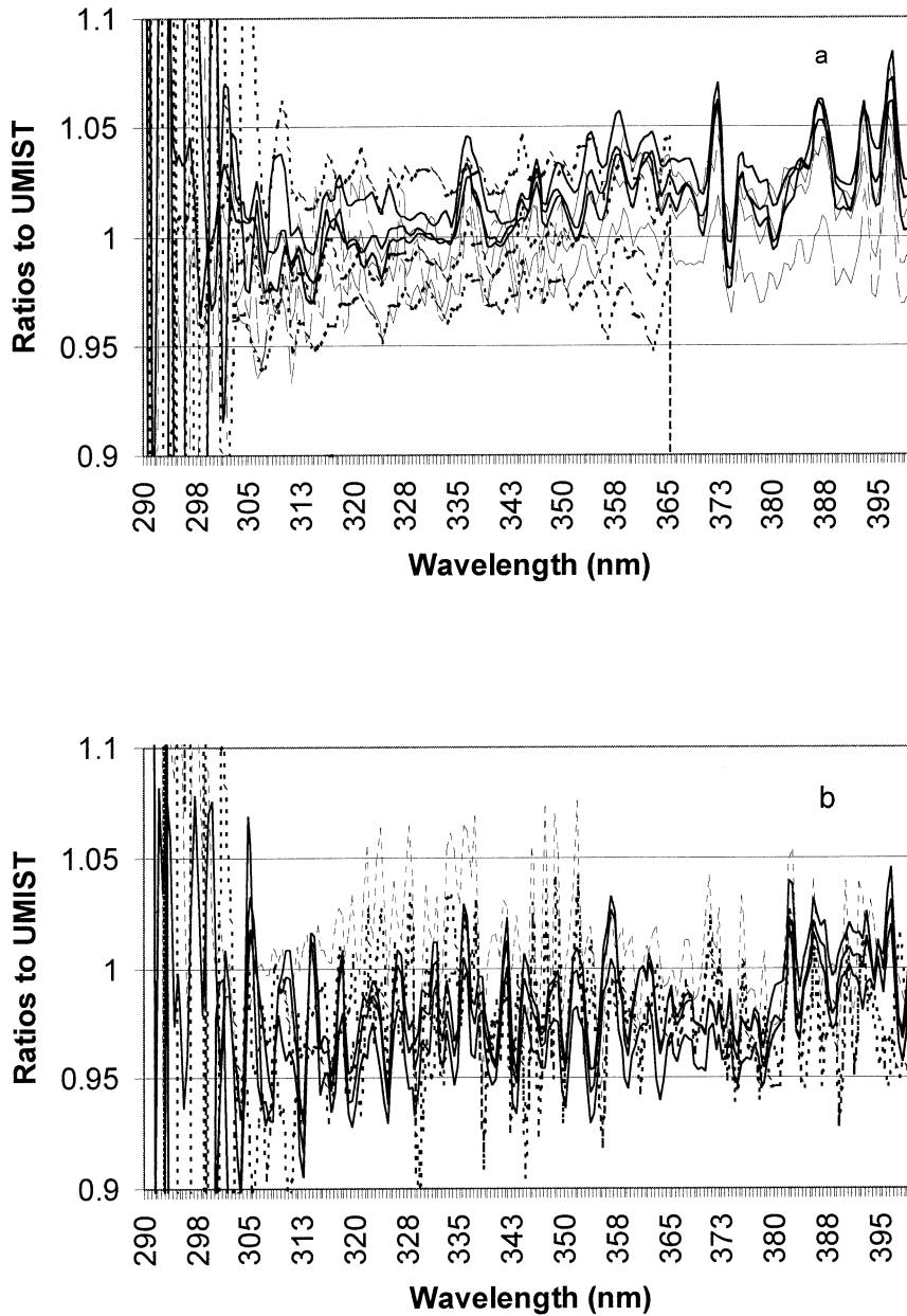
FIG. 2. Results of the three stability checks on day 222 expressed as a ratio of each instrument to the UMIST measurement for (a) global irradiance at SZA of 71°, 24°, and 64° (UIIMP, solid lines; AUTH, dotted lines; IFU, dashed lines) and (b) actinic flux at SZA of 66°, 24°, and 70° (IFU, solid lines; METCON, dotted lines).
