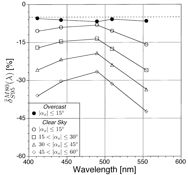
FIG. 7. The distribution of the average RPD values between the M80 and S95 methods, denoted \bar{\delta}_{S95}^{M80}(\lambda) . The results are split into clear-sky (open symbols) and overcast (solid symbols) conditions, and derived from 81 casts for the former and 19 casts for the latter. The dashed line represents an average underestimation of M80 with respect to S95 of -5\% .
