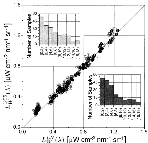
FIG. 8. The intercomparison of above- and in-water estimates of L_W(\lambda) during clear-sky conditions. The former are derived from the LoCNESS data, L_W^{LN}(\lambda) , and the latter using SeaSAS data with the S95 method plus the bidirectional ( Q -factor) correction L_W^{Q95}(\lambda) . The inset panels show the histograms of the absolute RPD values between the above- and in-water methods for uncorrected versus corrected data, |\delta_{LN}^{S95}(\lambda)| (upper-left light bars) and |\delta_{LN}^{Q95}(\lambda)| (lower-right dark bars), respectively. The total dataset is composed of 49 simultaneous casts which are separated into two groups (14 and 35 casts, respectively): |\alpha_s| \leq 15^\circ (solid circles), and |\alpha_s| > 15^\circ (open circles); the numerals within the symbols follow the wavelength convention of Fig. 4.
