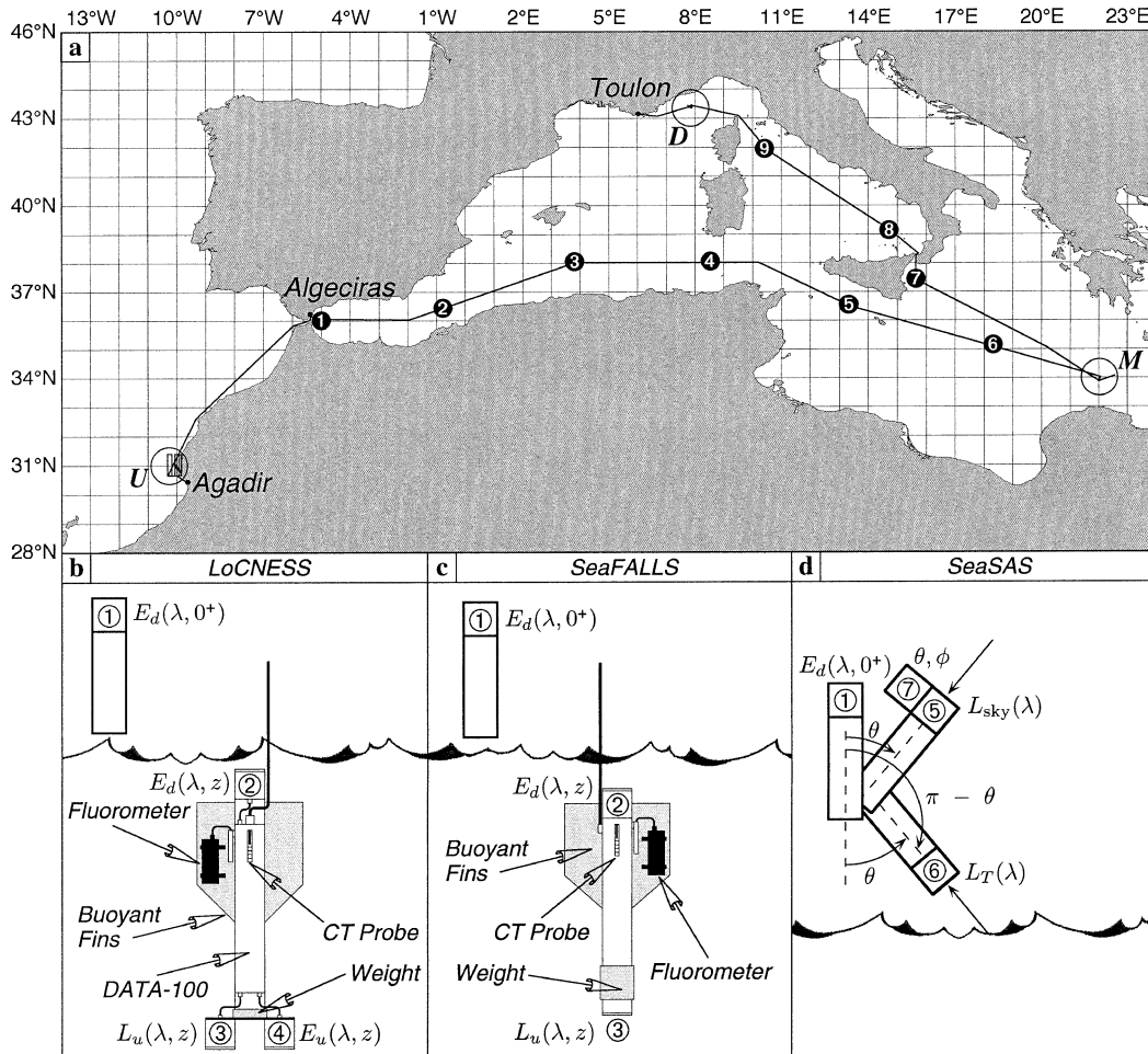
FIG. 1. A schematic of the PROSOPE cruise sampling: (a) the cruise track, with the short daily stations given by the (darkened) numbered bullets and the long multiday stations by the large circles (as encoded in Table 2); and the (b) LoCNESS, (c) SeaFALLS, and (d) SeaSAS instruments. For the latter, the (open) numerical bullets identify common sensor types. All three measurement systems were equipped with sensors to measure the vertical tilt \varphi of the radiometers during sampling.
