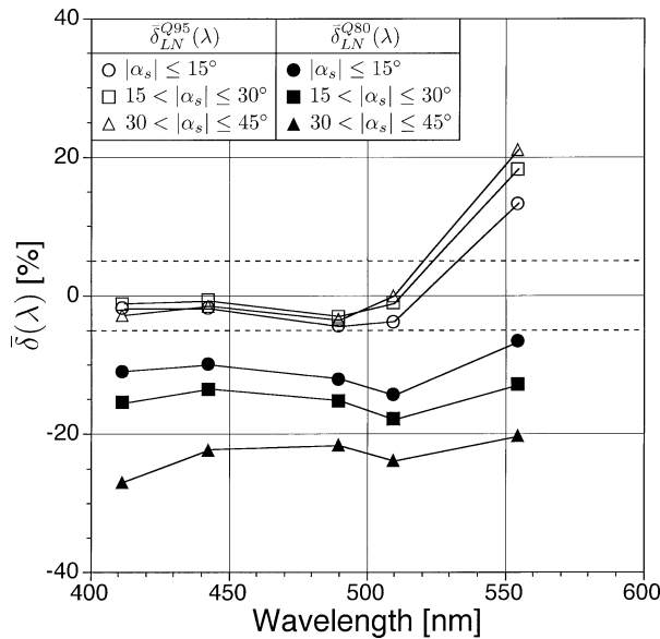
FIG. 10. A comparison of average RPDs between simultaneous in-water estimates of L_w(\lambda) (from LoCNESS) and above-water estimates corrected for bidirectional effects Q80 (solid symbols) and Q95 (open symbols), as a function of |\alpha_s| during clear-sky conditions (49 casts). The dashed lines indicate the \pm 5\% difference limits.
