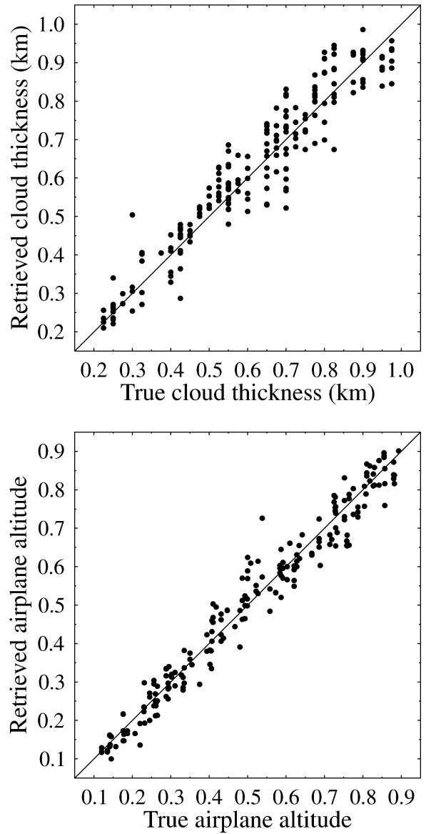
FIG. 11. The in situ lidar cloud thickness retrievals vs the (top) true thickness values and (bottom) retrieved vs true cloud airplane altitude. The airplane altitude is in terms of the fraction from cloud base to top. The 200 cases from the simulation used to test the neural network are shown. The quantization in true cloud thickness is due to the 25-m spacing of the simulated cloud layers.
