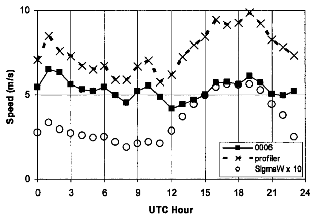
FIG. 1. Average peak wind speed values from the 60-m level of an acoustic profiler (x) and from the nearest corresponding level (62 m) of a nearby tall wind tower (■). The standard deviation of vertical velocity (o), multiplied by 10 and obtained from the vertical beam of the profiler, is also shown. Local time is given by the UTC hour minus 4.
