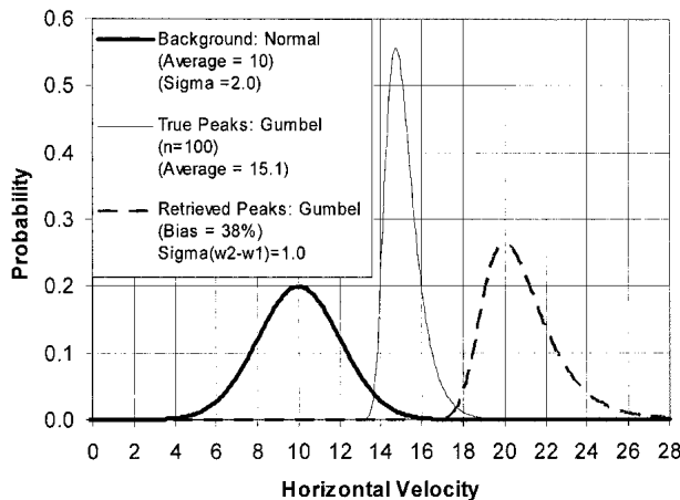
FIG. 3. Modeled PDFs of horizontal velocities illustrating Gumbel distributions of true and retrieved peaks derived from a background distribution that is Gaussian. Distribution parameters have been chosen to give an average background velocity of 10, an average value of 15.1 for the true peaks, and a bias of 38% for the retrieved peaks. The standard deviation of true horizontal velocities is 2.0 and that of the residual vertical velocity is 1.0.
