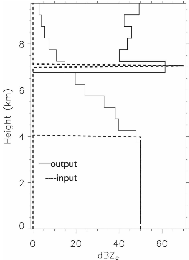
FIG. 5. Additional simulations of synthetic Z_e profiles according to the algorithm in Fig. 1. The first input profile corresponds to a layer of enhanced Z_e at a particular height (thick dashed line; a 70-dBZ layer at a 7-km height). The second input profile corresponds to a region of enhanced, constant Z_e below a particular height (thin dashed line; a 50-dBZ region below the 4-km level). The thick (thin) stepped line is the output \bar{Z}_e profile for the first (second) input profile.
