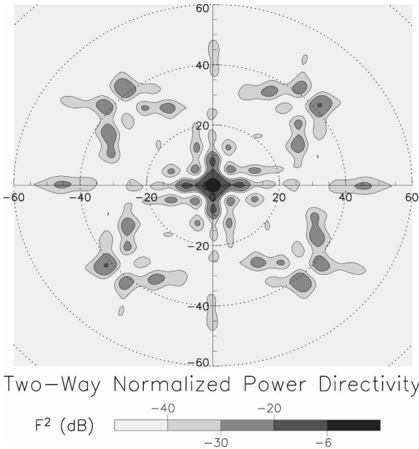
FIG. 3. Two-way antenna pattern (also known as a polar diagram, F^2 ) for the McGill VHF radar. The concentric circles correspond to the zenith angles in the x and y axes. The azimuth angles start clockwise from the positive y axis. Geographic north is located at 48.7^\circ azimuth.
