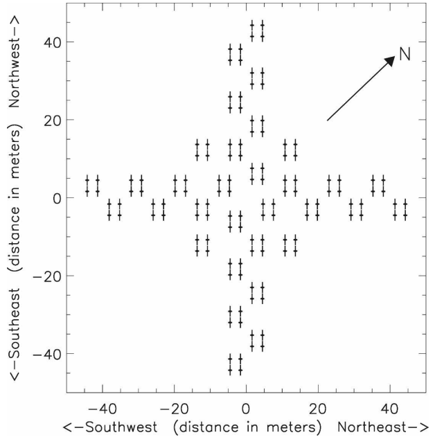
FIG. 2. Plan for the antenna array of the McGill VHF radar. Note that the aerials are aligned at 48.7^\circ from the north.
