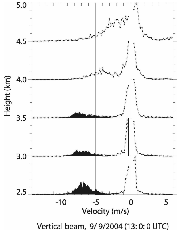
FIG. 7. Vertical profile of reflectivity-factor densities observed by the McGill VHF radar at 1300 UTC 9 Sep 2004. The dotted lines correspond to raw Doppler spectra, and the dark areas below each spectrum correspond to the precipitation signal, according to the algorithm described by Campos et al. (2007). These dark areas relate to the rain Z_e values plotted as dotted lines in Fig. 6. Vertical lines are drawn at the spectral bins corresponding to the clear-air vertical velocities. Above a 3.5-km height, the precipitation is in the solid or melting phase, and the precipitation spectra merge with the clear-air spectra.
