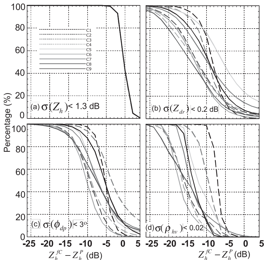
FIG. 12. Same as in Fig. 10, but showing the amount of data in percentage meeting the precision threshold for all nine ground clutter types indicated by different line styles and colors [scale in panel (a)].
