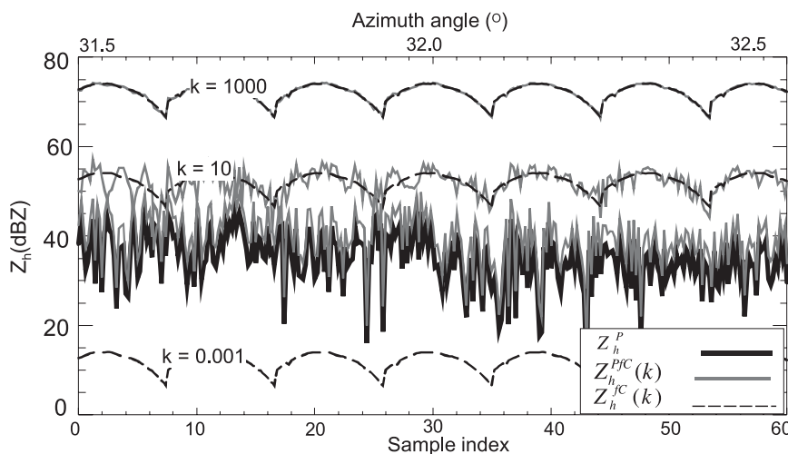
FIG. 6. Same as in Fig. 5c, but showing all intensity-modified ground clutter C1 for k = 0.001 , 10, and 1000 [ Z_h^{IC}(k) ; dashed black lines] and the superposition of precipitation and the intensity-modified ground clutter [ Z_h^{PIC}(k) ; solid gray lines]. Horizontal reflectivity of precipitation is denoted as Z_h^P and indicated as a solid black line.
