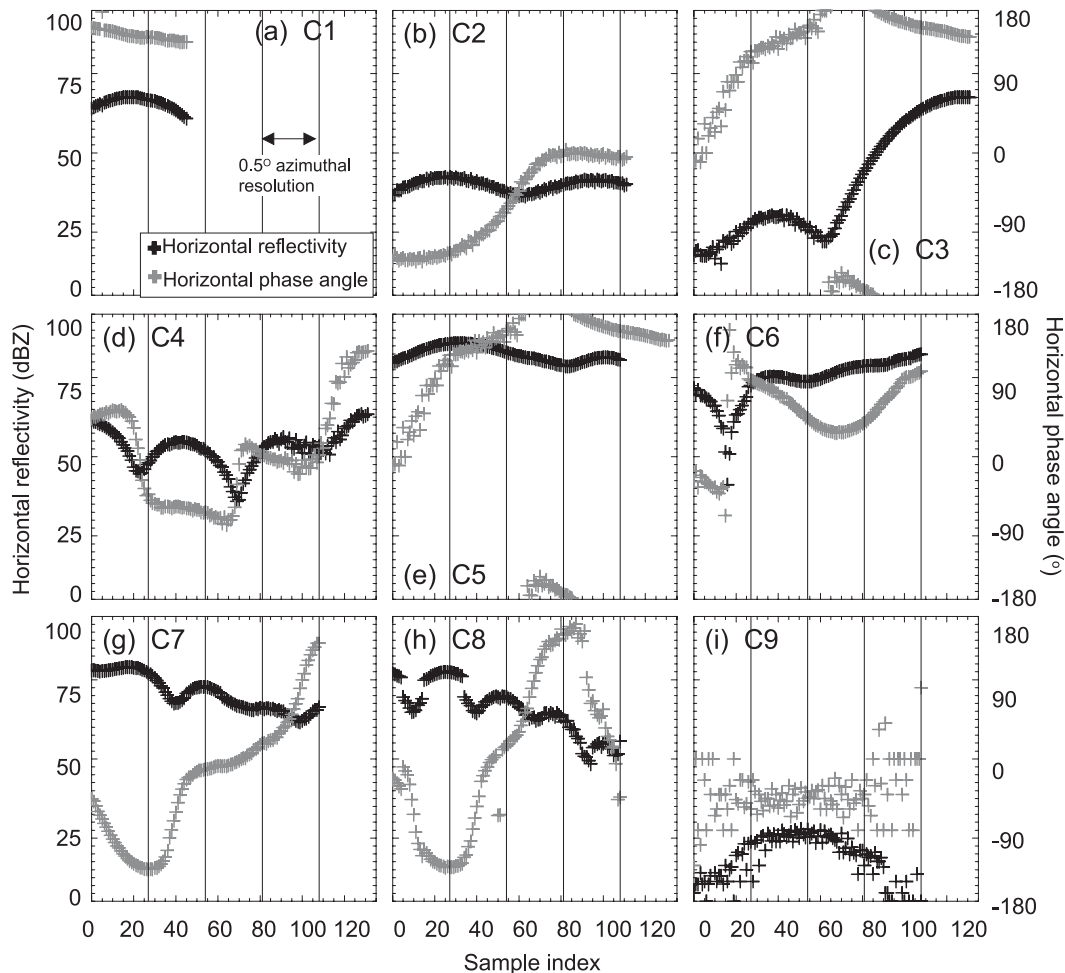
FIG. 3. Same as in Fig. 2, but showing horizontal reflectivity (black plus symbols) and phase angle (gray plus symbols) of nine urban obstacles denoted as (a)–(i) C1, C2, C3, . . . , C9, respectively. Radial position, azimuthal range, and mean values of the polarimetric quantities are listed in Table 2.
