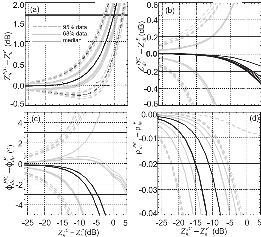
FIG. 9. Median (solid black lines), 68% of the data (solid gray lines), and 95% of the data (dashed gray lines) for (a) horizontal reflectivity, (b) differential reflectivity, (c) differential phase, and (d) correlation coefficient as a function of the difference between intensity-modified ground clutter and precipitation for all eight analysis times on 15 Nov and 2–3 Oct 2006, including all ground clutter types. The number of members per clutter intensity class is listed in Table 5. Precision thresholds are indicated as black horizontal lines.
