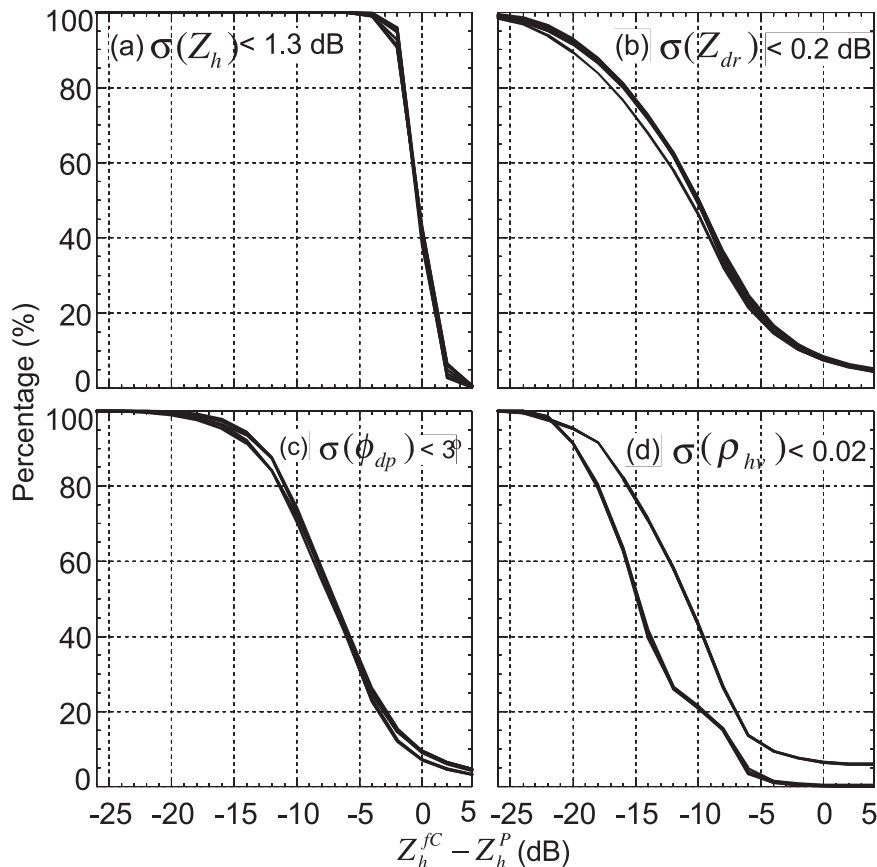
FIG. 10. Amount of data in percent for (a) Z_h , (b) Z_{dr} , (c), \phi_{dp} , and (d) \rho_{hv} that meets the predefined precision thresholds. The solid, black lines represent the eight analysis times on 15 Nov and 2–3 Oct 2006, including all ground clutter types.
