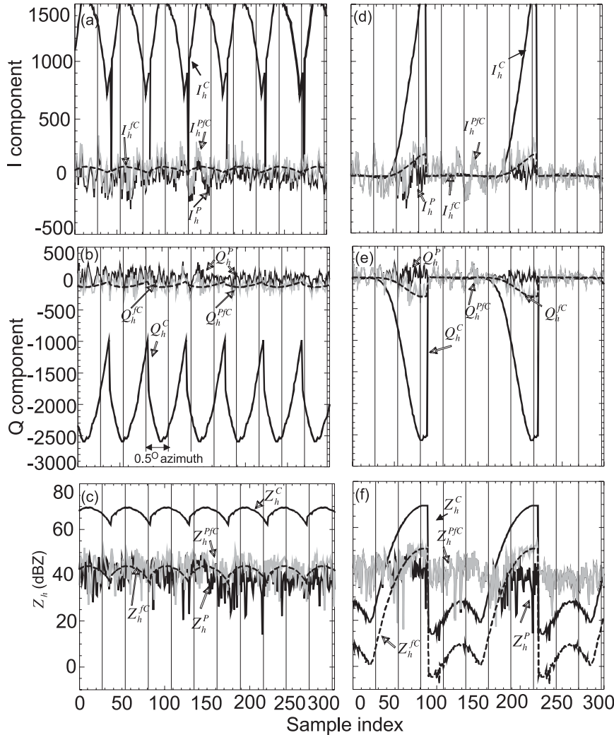
FIG. 5. Superposition of precipitation at 1451 UTC 15 Nov 2005 and ground clutter type (a)–(c) C1 and (d)–(f) C3. (a), (d) In-phase component ( I_h ); (b), (e) quadrature component ( Q_h ); and (c), (f) reflectivity at horizontal polarization ( Z_h ) are shown. Observed precipitation denoted as superscript P and ground clutter denoted as superscript C are indicated as solid black lines, respectively. Intensity-modified ground clutter [ k = 1 in Eq. (1)] denoted as superscript fC is indicated as dashed black line. The superposition of precipitation and intensity-modified ground clutter denoted as superscript PfC is indicated as solid gray line.
