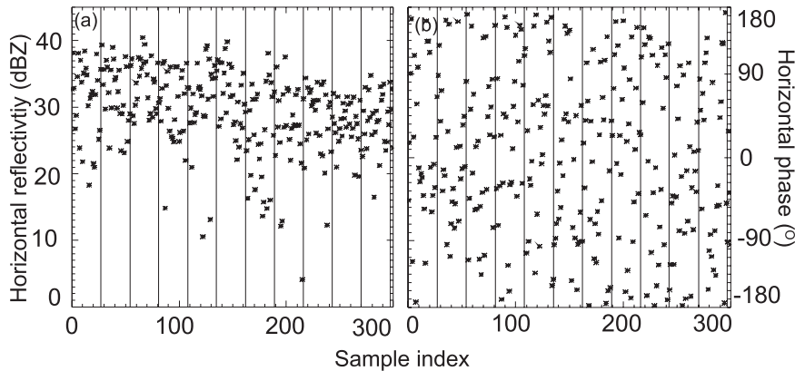
FIG. 2. Distribution of (a) horizontal reflectivity and (b) horizontal phase angle of moving scatterers primarily related to rain along an azimuthal interval of \sim 5.5^\circ at 67.4-km range at 1451 UTC 15 Nov 2005. Each symbol represents an I and Q measurement at horizontal polarization. For an azimuthal resolution of 0.5^\circ indicated by thin vertical lines, 27 successive samples were averaged.
