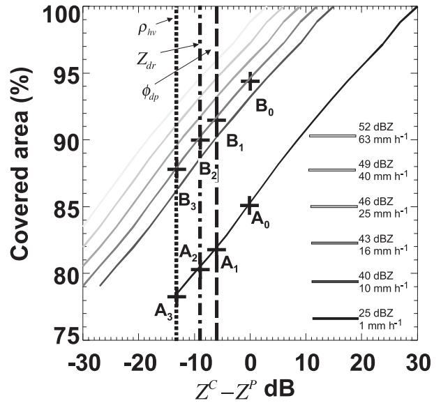
FIG. 14. Spatial coverage of the measurement domain obtained by the three Swiss weather radars as indicated in Fig. 1 as a function of Z_h^C - Z_h^P for rainfall intensities indicated by gray lines ranging from 1 to 63 mm h -1 . To have the measurement precision, precipitation magnitude should exceed ground clutter magnitude by 6 dB as indicated as dashed line for \phi_{dp} , 9 dB as indicated as dashed–dotted line for Z_{dr} , and 13 dB as indicated as dashed–dotted line for \rho_{hv} .
