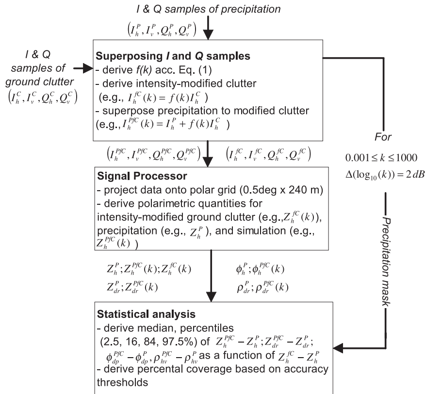
FIG. 4. Schematic showing the three steps of the data processing chain discussed in section 3.
