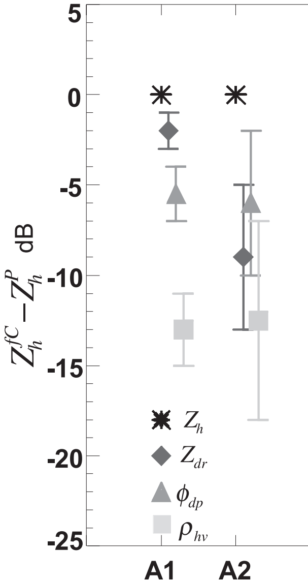
FIG. 13. Minimum and maximum values of Z_h^{fC} - Z_h^P indicated by error bars and their mean indicated by the symbols for medians of analysis 1 (denoted as A1) and analysis 2 (denoted as A2). Star symbols represent Z_h , diamond symbols represent Z_{dr} , triangle symbols represent \phi_{dp} , and square symbols represent \rho_{hv} .
