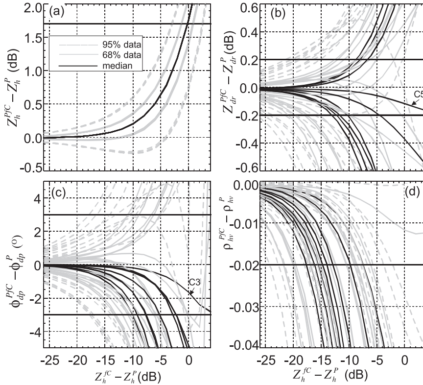
FIG. 11. Same as in Fig. 9, but showing median and percentiles of nine ground clutter types, including all precipitation events in the analysis. Median of ground clutter (b) type C5 is highlighted as is (c) type C3.
