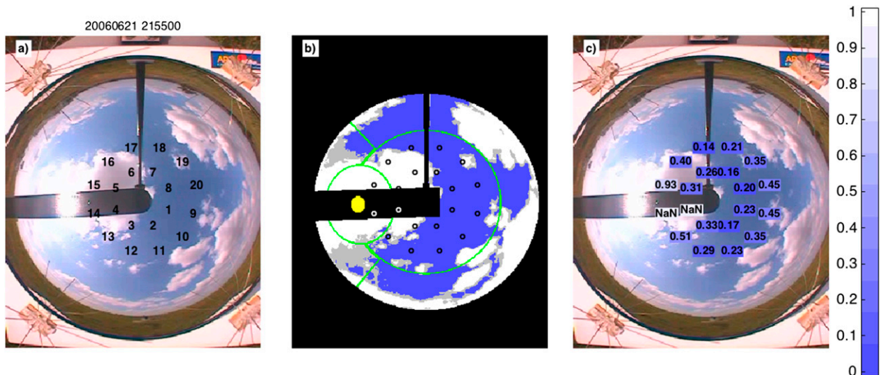
FIG. 3. TSI 2155 UTC 21 Jun 2006. (a) The locations of the 20 spots sampled from the TSI images to create synthetic ceilometer observations, overlaid on a raw TSI image. (b) The TSI cloud mask image product, with blue, gray, and white indicating clear, thin, and opaque clouds, respectively. The green circle around zenith indicates a 100° FOV, and the green circle around the sun indicates a 25° radius. (c) The sky cover fraction averages at the 20 synthetic ceilometer locations, valid for the 30-min period leading up to this image. Spots 4 and 5 and 13–16 lie within 35° of the sun circle. The TSI-calculated hemispheric sky cover is 0.226, whereas the sky cover fraction of synthetic ceilometers beyond 35° of the sun circle range from 0.14 to 0.45 with a mean of 0.272.
