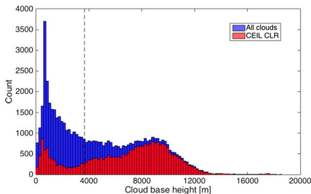
FIG. 7. Histogram of cloud-base height determined by the MPL corresponding to all observations (blue) and observations where the ceilometer observes only clear (0–0.05) skies (red). Mean cloud-base height was obtained by averaging the lowest cloud base as observed by the MPL over a 30-min period with the last 10 min double weighted in order to be consistent with sky cover observations. The vertical dashed line at an altitude of 3660 m corresponds to the upper limit of operational ceilometer observations.
