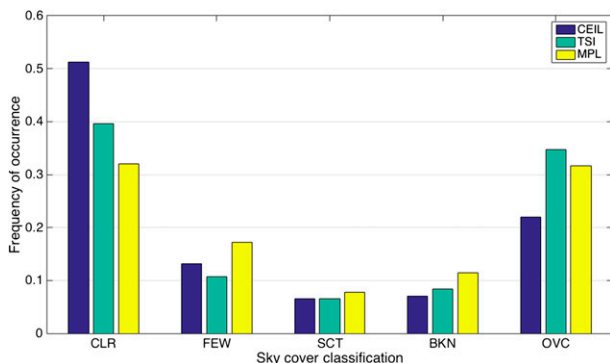
FIG. 2. A climatology of cloudiness as observed at the SGP site for the three instruments analyzed in this work: CEIL (blue), TSI (teal), and MPL (yellow), sorted into the operational sky cover classification bins. Because of limitations of the MPL dataset, this climatology covers only the period between August 2006 and December 2012.
