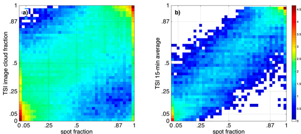
FIG. 4. Joint histograms of all 20 synthetic ceilometers compared with TSI hemispheric observations. (a) The instantaneous TSI image over the whole-sky dome, corrected for haze following Long (2010). There are a total of 429 150 observations and an RMSE of 0.161. (b) The 15-min average of TSI images in a 100° FOV is compared to the spot cloud fraction, after removal of spots that occur within 35° of the sun circle, observations prior to 9 Aug 2006, and observations where the lowest cloud base determined by the MPL is above 3660 m. There are a total of 92 614 observations and an RMSE of 0.0860. Note the logarithmic color scale applies to both panels.
