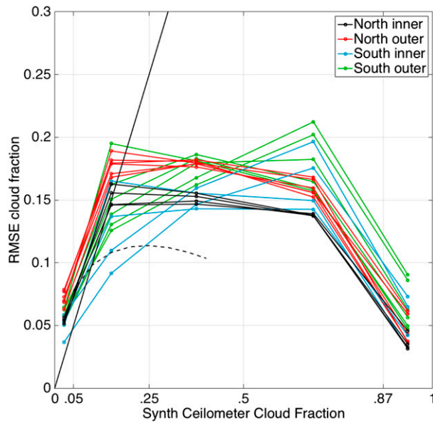
FIG. 6. The RMSE between the synthetic ceilometer observations and the 15-min averaged 50^\circ TSI cloud fraction for each ceilometer cloud fraction class. Dashed line is from Eq. (10) in Berg and Stull (2002), while the solid line is a 1:1 fit; points above the solid line have a greater variability than the signal.
