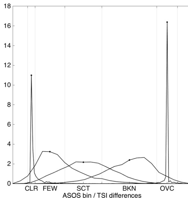
FIG. 5. The probability distributions of the difference (TSI minus synthetic ceilometer) for each of the ASOS bins of sky cover. Note that the clear and overcast distributions have been reduced by a factor of 5 for visibility. The center of each distribution (representing perfect agreement) is indicated with a dot.
