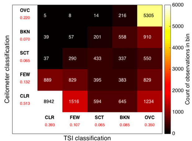
FIG. 1. Intercomparison of sky cover classification as observed by the TSI and the CEIL. The number of observations in each bin is shown, and bins are colored according to the number of observations following the color scale on the right-hand side of the image. Red numbers below each bin identifier represent the fraction of cloud cover classifications observed by each instrument. The color scale is capped at 6000 observations to enhance contrast between intermediate bins.
