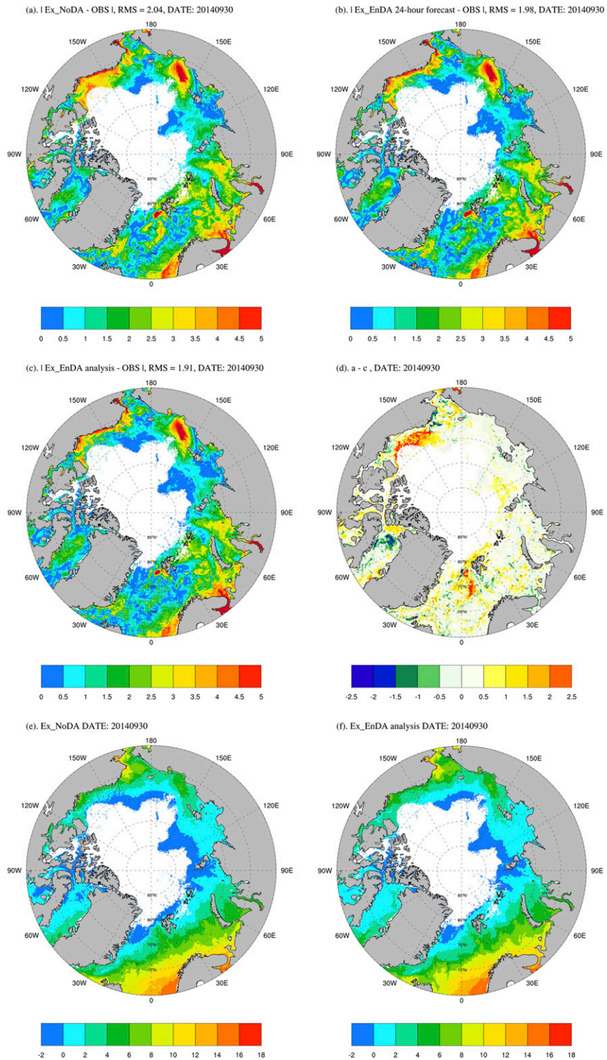
FIG. 5. As in Fig. 3, but for 30 Sep 2014.
