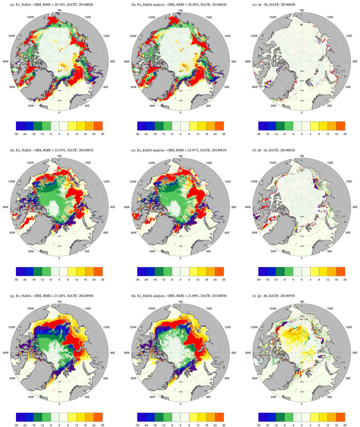
FIG. 7. Deviation (%) between modeled SIC and AMSR2 SIC data. (top) 20 Jun 2014, (middle) 10 Aug 2014, and (bottom) 30 Sep 2014. (left) Ex_NoDA, (center) Ex_EnDA analysis, (right) improvement (absolute difference: left column minus center column).
