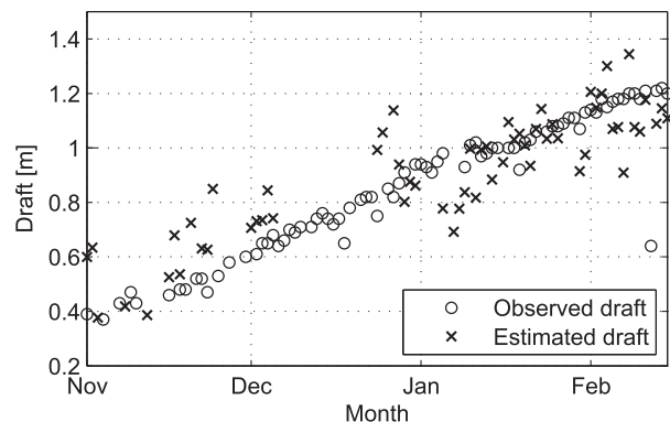
FIG. 11. Time series of in situ mode draft (circles) and estimated draft calculated from Eq. (6) using filtered GR(18V, 36V) values (crosses).
