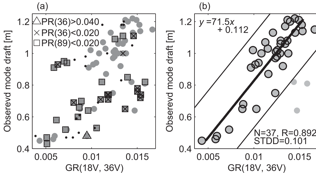
FIG. 10. (a) Scatterplots of unfiltered GR(18V, 36V) vs daily mode draft in the period from November to mid-February. Points with triangles, crosses, and squares indicate contaminated data identified by the maximum and minimum thresholds of PR(36) and the minimum threshold of PR(89) listed in Table 1, respectively. Black points indicate data eliminated by normalized moments of draft probability distributions or the minimum threshold of SIC. (b) Scatterplot of filtered GR(18V, 36V) vs daily mode draft. The thick line is the fitted line of Eq. (6) derived from data at the gray points edged with black lines. The adjacent thin lines represent 1.5 standard deviations of differences of the points from the fitted line.
