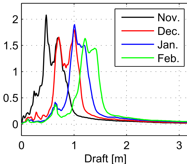
FIG. 5. Monthly draft probability distributions binned into 1-cm intervals in November–February.
