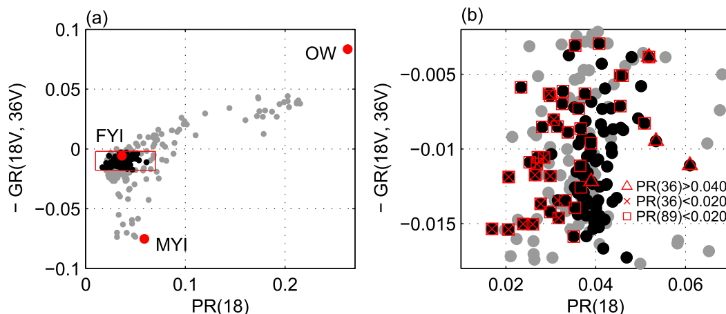
FIG. 7. (a), (b) Scatterplots of PR(18) vs GR(18V, 36V). Tie points for MYI, FYI, and open water are indicated by red points in (a). The area within the red box in (a) is enlarged in (b). Points with red triangles, crosses, and squares indicate contaminated data identified by the maximum and minimum thresholds of PR(36) and the minimum threshold of PR(89) listed in Table 1, respectively.
