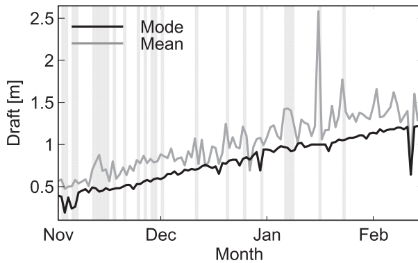
FIG. 6. Time series of daily mode and mean draft values (black and gray lines, respectively). The gray shaded regions indicate times with daily draft probability distributions showing multiple sea ice modes. The multiple sea ice modes are identified by normalized moments of the draft probability distributions above 0.6.
