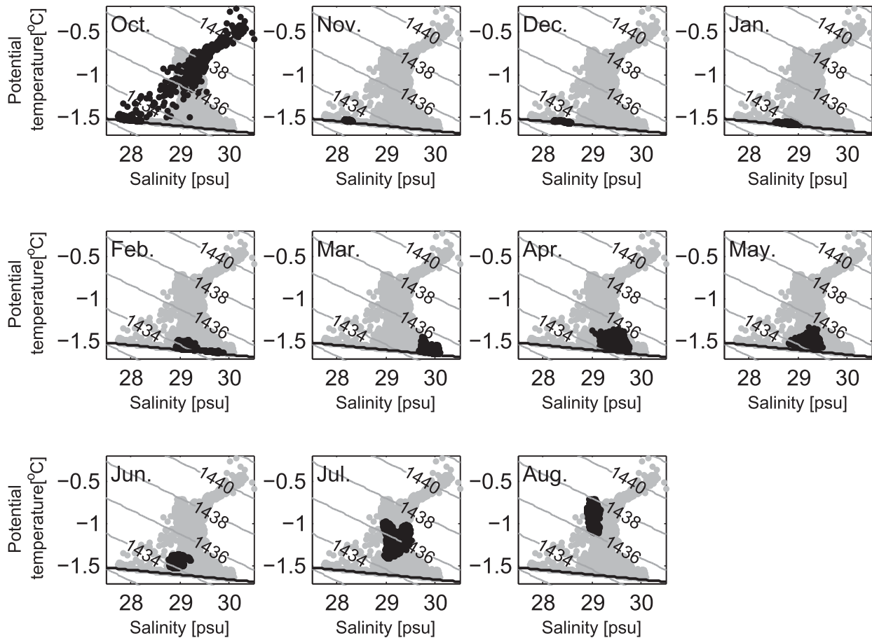
FIG. 3. Monthly scatterplots of potential temperature vs salinity obtained from moored CTD observations at approximately 25 m. Data in each month are plotted using black points, and all available data in October–August are plotted using gray points. Black lines represent freezing temperatures. Gray contours are isolines of sound speeds.
