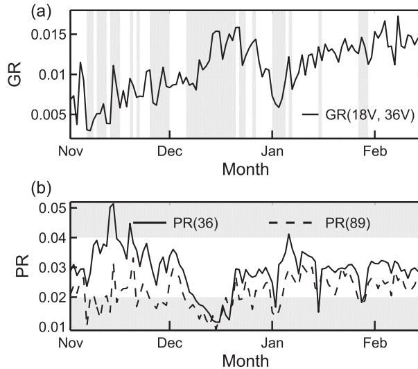
FIG. 8. (a) Time series of GR(18V, 36V) at the mooring site. The gray shaded regions indicate times with contamination effects in brightness temperature data identified by the maximum and minimum thresholds of PR values listed in Table 1. (b) Time series of PR(36) and PR(89) shown by solid and dashed lines, respectively. PR values in the gray shaded regions are above (below) the maximum (minimum) threshold.
