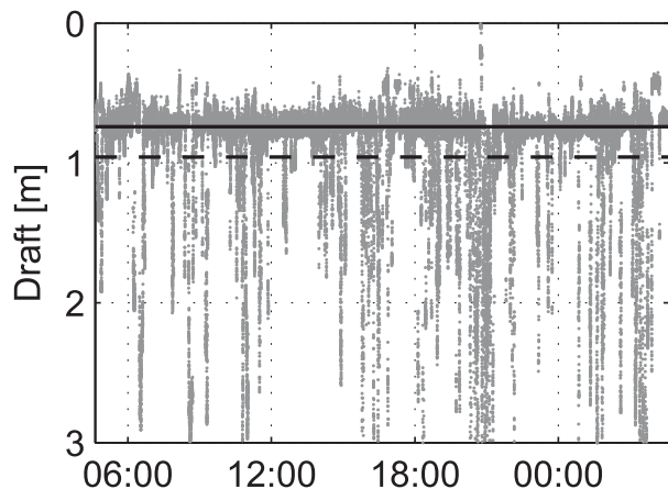
FIG. 4. Time series of IPS-measured draft recorded at 1-s intervals (gray points) compared with the daily mode and mean draft (solid and dashed lines, respectively) on 16 Dec 2014.
