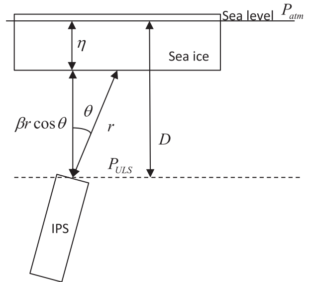
FIG. 2. Schematic showing IPS measurements used to calculate sea ice draft.
