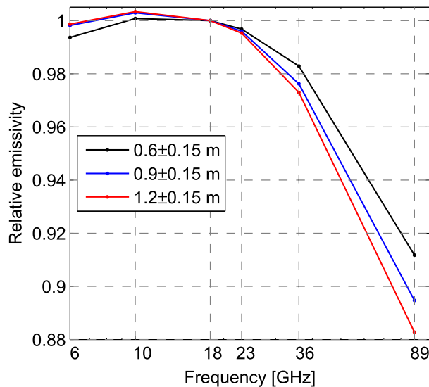
FIG. 9. Relative emissivities calculated from filtered brightness temperature data in vertical polarizations plotted vs AMSR2 frequencies. The emissivities at each frequency are binned into three values of the daily mode draft, 0.6 \pm 0.15 , 0.9 \pm 0.15 , and 1.2 \pm 0.15 m (black, blue, and red lines, respectively). See the text for a further description of the relative emissivities.
