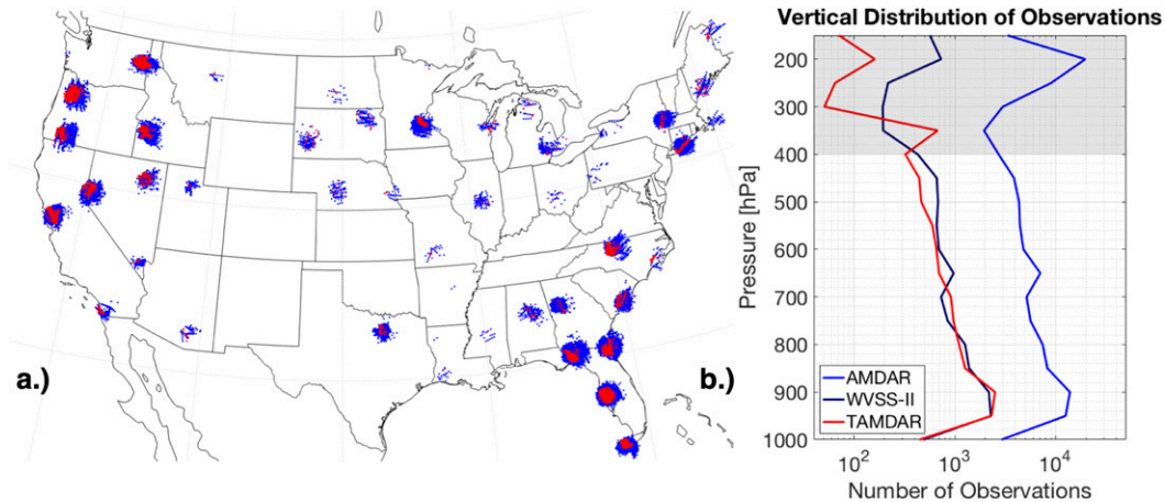
FIG. 1. (a) Map of the locations of radiosonde observations with AMDAR/WVSS observations (blue) and TAMDAR observations (red) between the surface and 400 hPa and (b) vertical profile of the number of observations collocated with radiosondes for the study period from AMDAR (blue), WVSS (dark blue), and TAMDAR (red) per 50 hPa layer. Only observations from below 400 hPa were used in this study; observations from higher altitudes are included in (b) to illustrate the peak in AMDAR observations at cruising altitude but are shaded to denote their elimination from further use in this analysis.
