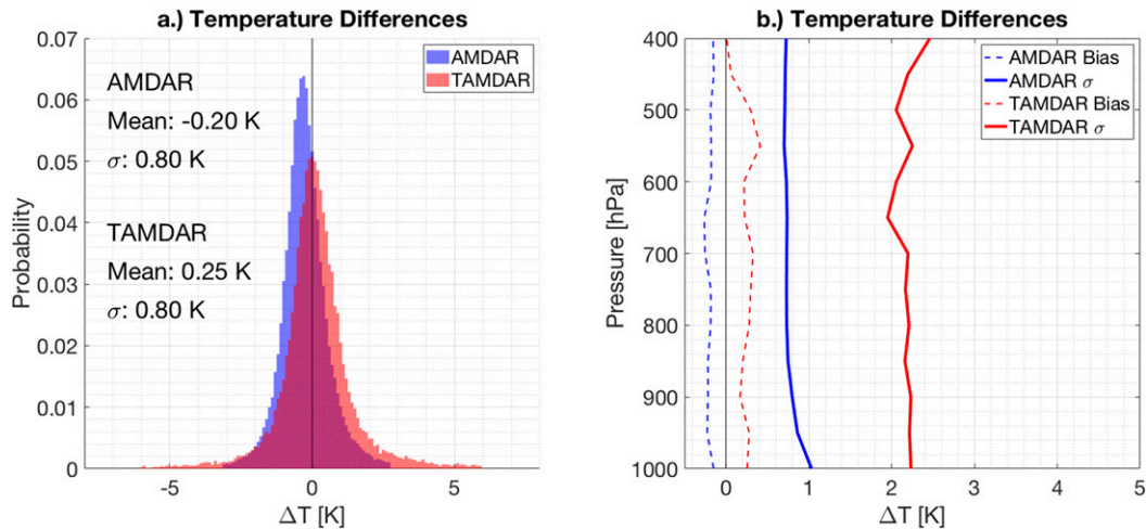
FIG. 4. (a) As in Fig. 2, but for temperature in 0.1 K bins. (b) As in Fig. 3, but for temperature (in K).
