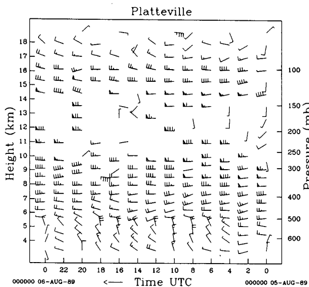
FIG. 11. Horizontal winds measured by the WPL VHF wind profiler at Platteville, Colorado, from 0000 UTC 5 August to 0000 UTC 6 August 1989 every other hour at 500-m height intervals.
