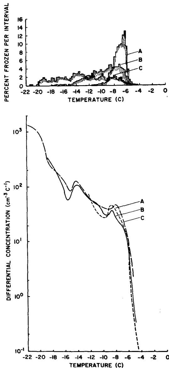
FIG. 4. Experimental results for three sets of runs with different sizes of drops, all from the same sample of a melted hailstone: A, 725 drops of 0.04 \text{cm}^3 each; B, 720 drops of 0.01 \text{cm}^3 each; and C, 704 drops of 0.0025 \text{cm}^3 each. The upper diagram is a histogram representation of the numbers of drops frozen per 0.27^{\circ}\text{C} interval, the lower diagram the corresponding spectra derived from (11).
